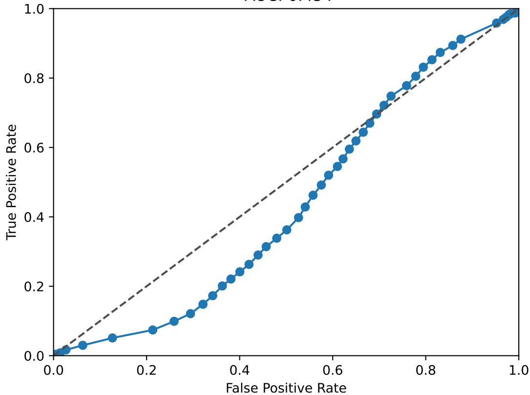
CUX2 ROC Curve AUC: 0.434
