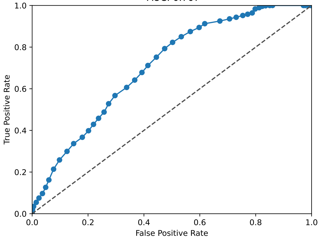
EGR1 ROC Curve AUC: 0.707
