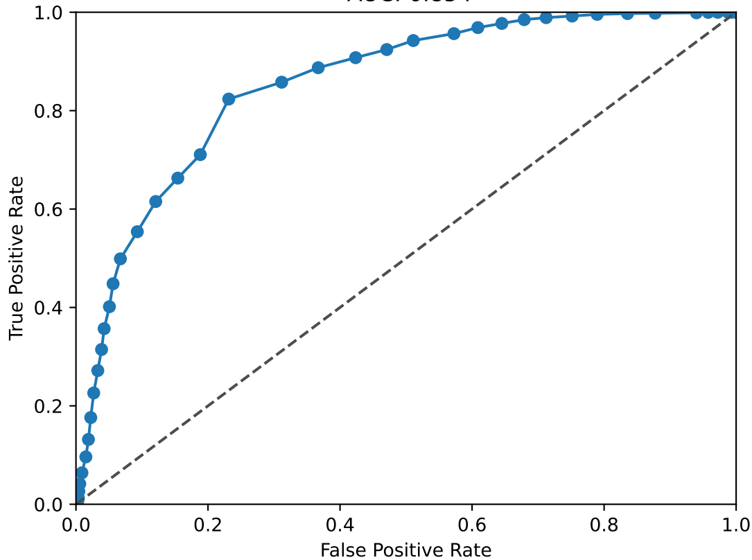
FOS ROC Curve AUC: 0.854
