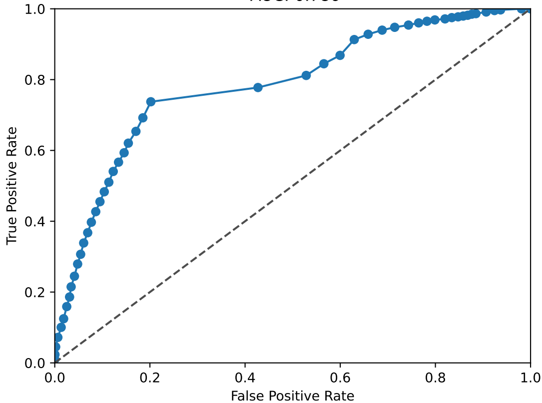
JUN ROC Curve AUC: 0.786
