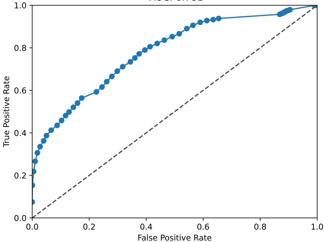
LMX1B ROC Curve AUC: 0.781
