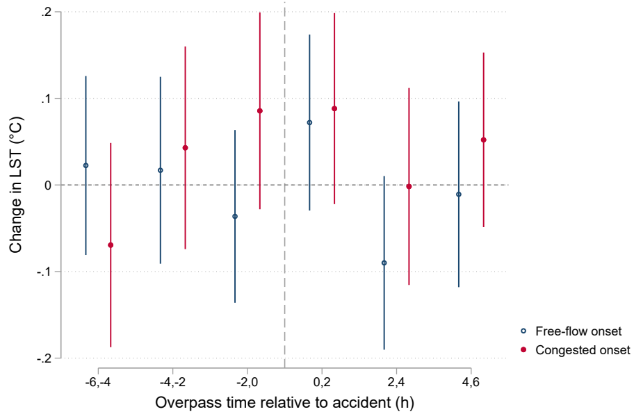
Figure 4: Event study by accident onset: surface temperature. Same specification as Figure 3, Y = \text{LST } (^\circ\text{C}) . Pre-accident leads are flat for both groups, consistent with the exclusion restriction.
