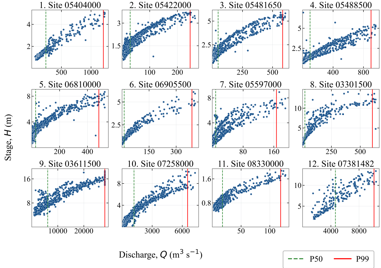
Figure 2: Observed stage–discharge rating curves for the 12 sites numbered in Figure 1.
