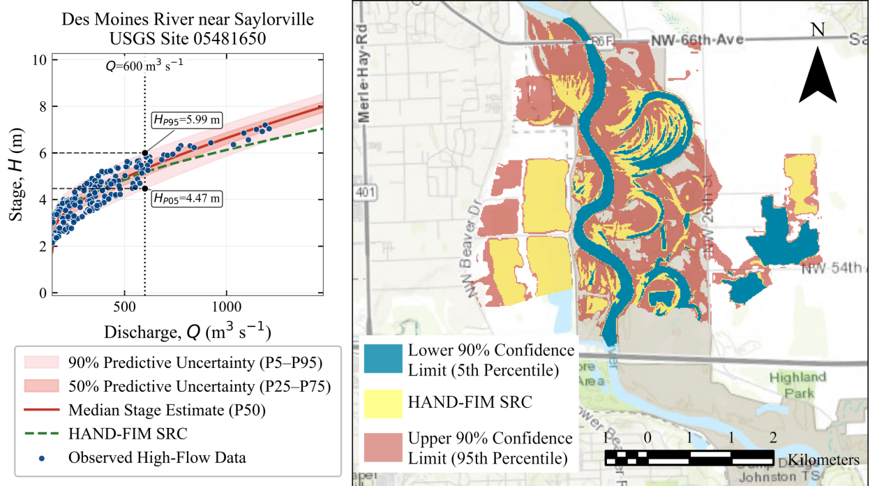
Figure 6: Des Moines River near Saylorville (USGS 05481650) at Q = 600 \text{ m}^3 \text{s}^{-1} . Left: probabilistic rating curve with the 5th/95th percentile stage estimates. Right: corresponding FIMs.
