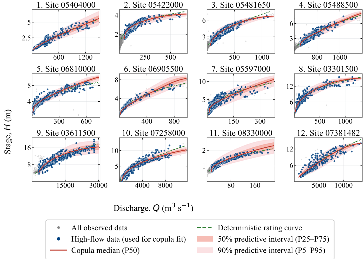
Figure 3: Probabilistic rating curves from the copula-based framework applied to representative IFMHA stations.
