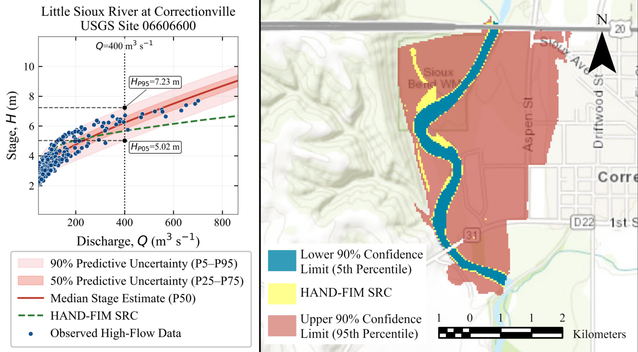
Figure 5: Little Sioux River at Correctionville (USGS 06606600) at Q = 400 \text{ m}^3 \text{ s}^{-1} . Left: probabilistic rating curve with the 5th/95th percentile stage estimates. Right: corresponding FIMs.
