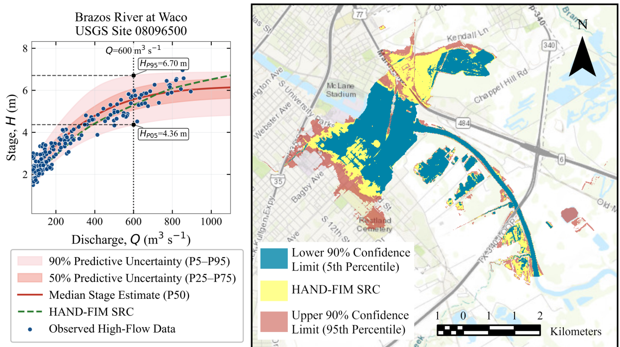
Figure 7: Brazos River at Waco (USGS 08096500) at Q = 600 \text{ m}^3 \text{s}^{-1} . Left: probabilistic rating curve with the 5th/95th percentile stage estimates. Right: corresponding FIMs.
