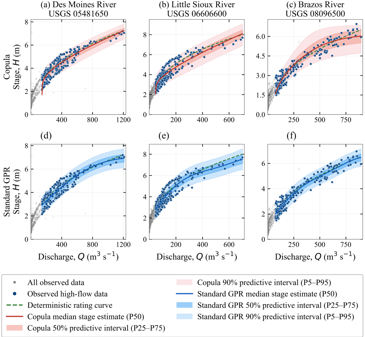
Figure 4: Probabilistic rating curves for the three case-study sites. First row: copula-based probabilistic rating curves; second row: GPR-based probabilistic rating curves.
