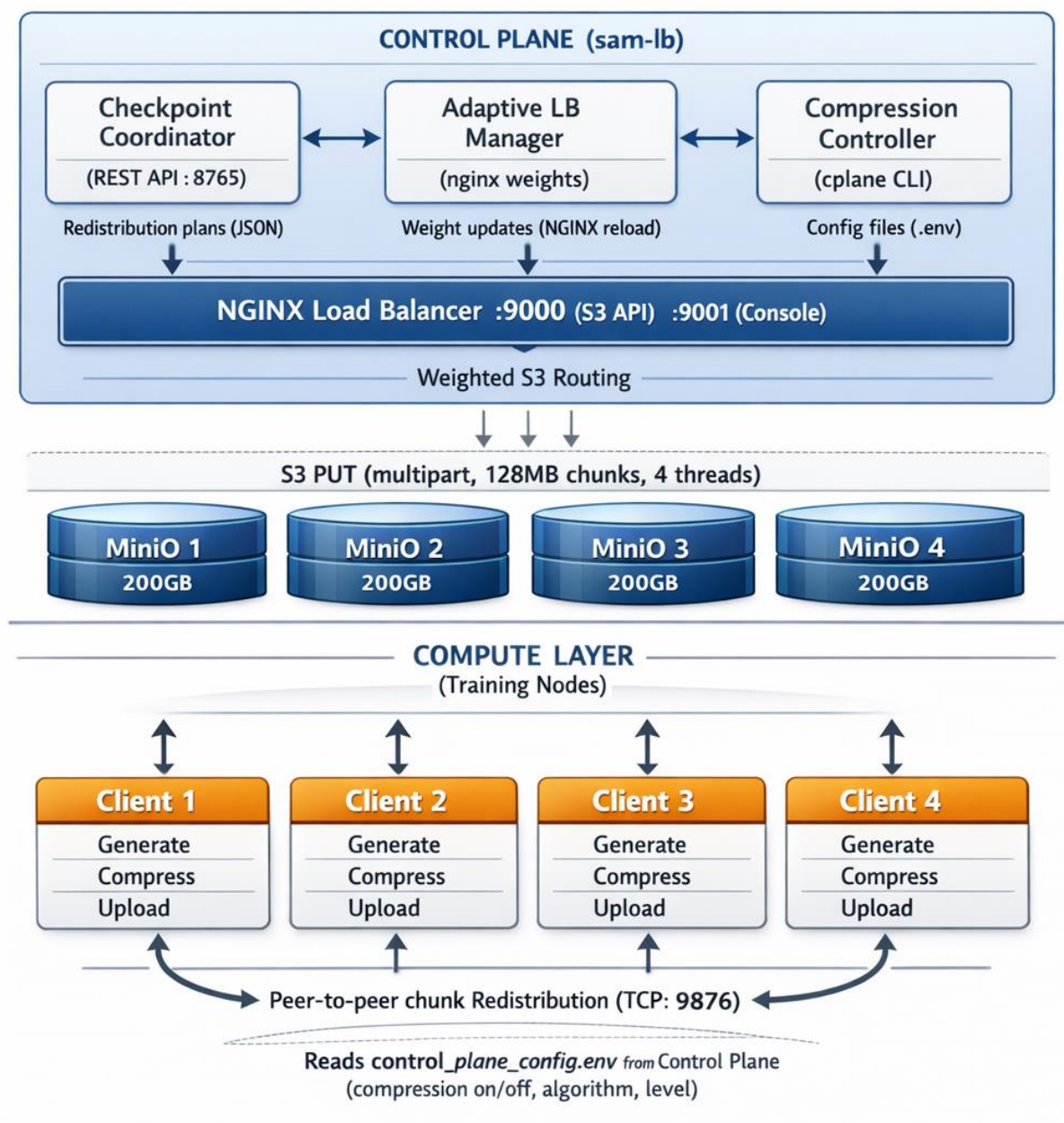
Figure 1. CPaaS architecture showing the control plane, storage layer, compute clients, and peer-to-peer redistribution path.
