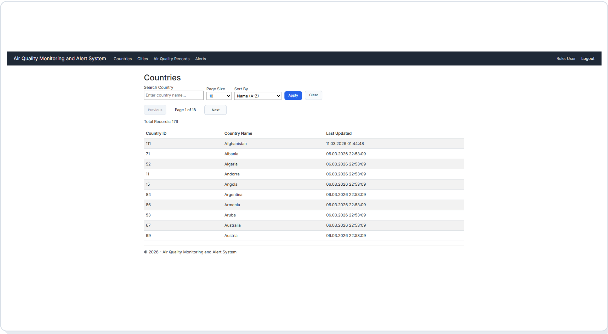
Countries page - search, sort and pagination for country records
