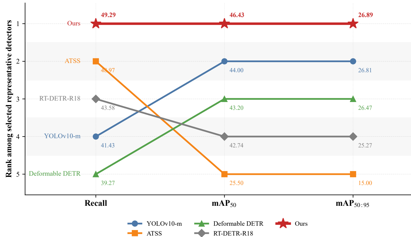
Ranking Flow of the Best Representative Models on VisDrone2019
