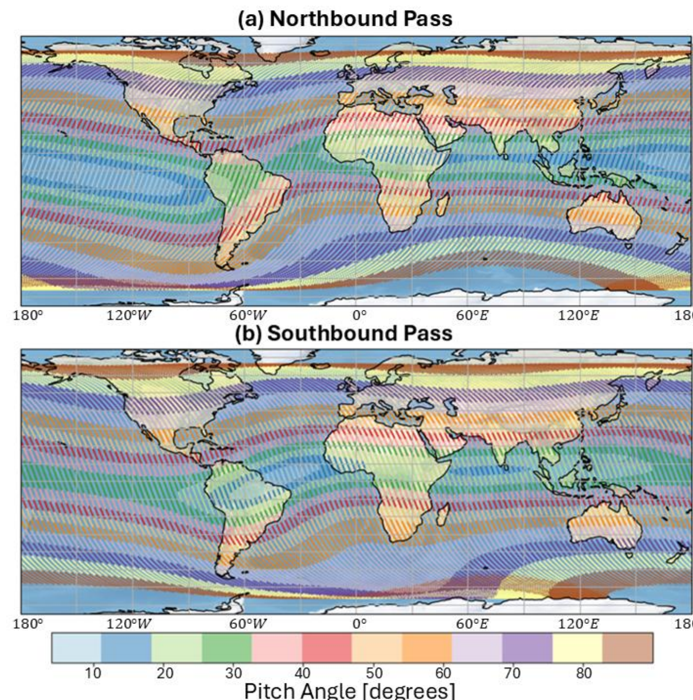
Figures 3: Example of the PAs sampled during (a) northbound and (b) southbound passages of a quiet month.
