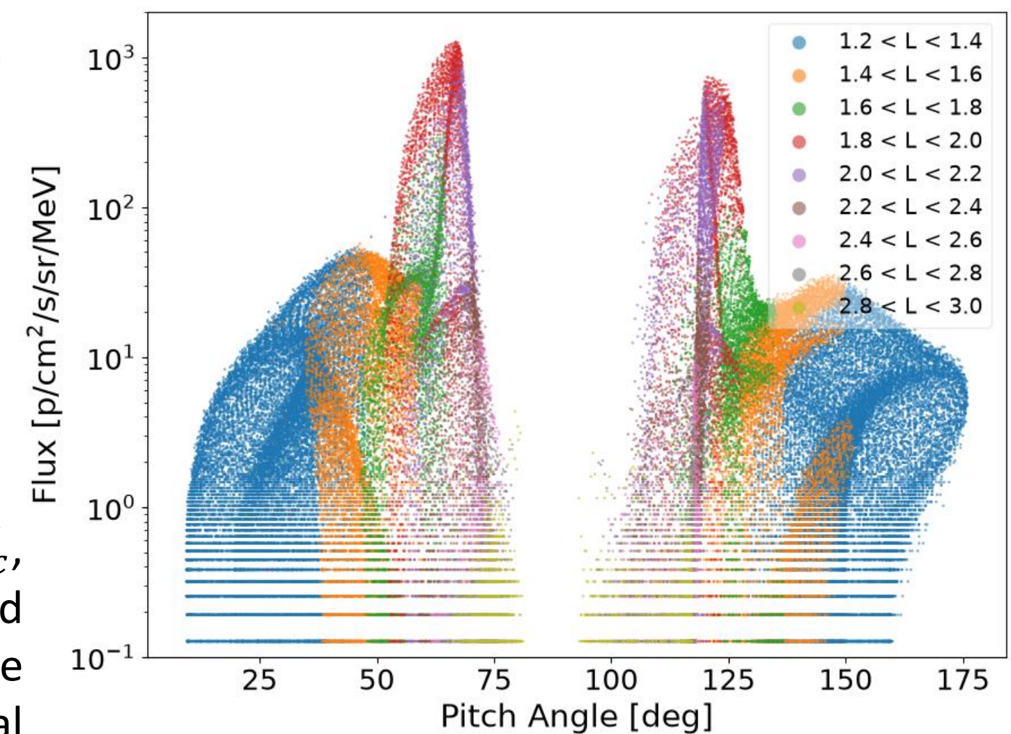
Figures 4: PAD of the measured proton fluxes at 9 MeV, where colour indicates the different L-shells.
