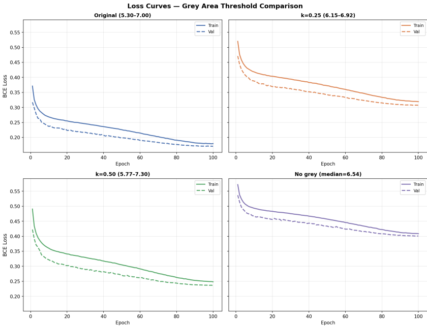
Figure 6.18: Comparison of training and validation loss between the thresholds ran on the same model
