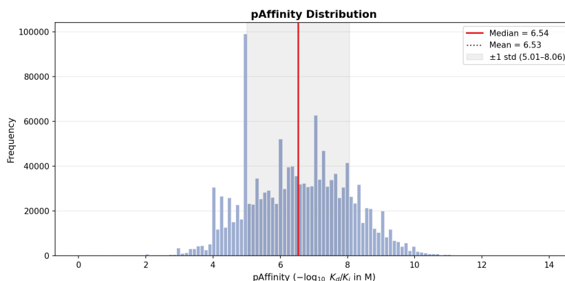
Figure 6.15: pAffinity distribution with median and mean marked
