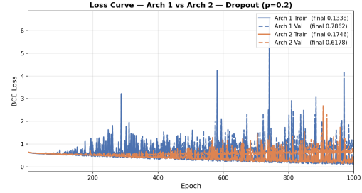
Figure 6.22: Loss curves comparing architecture Iteration 2 to architecture Iteration 1.
