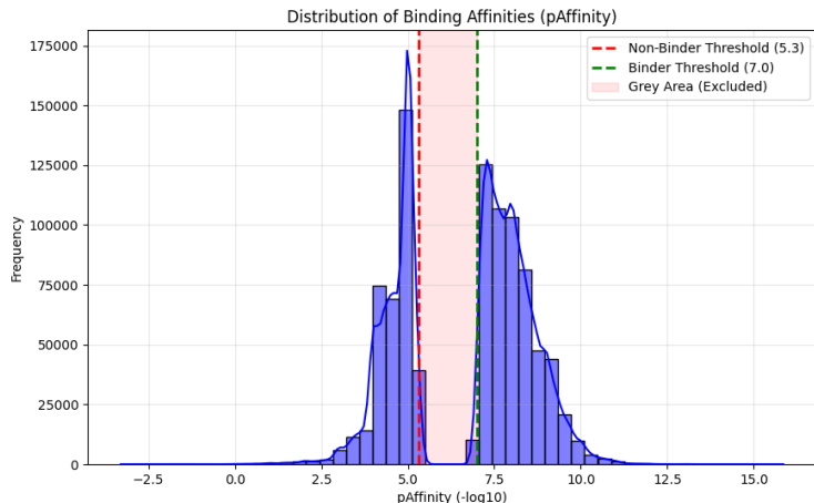
Figure 3.3: Distribution of pAffinity values in the filtered dataset. The red shaded region represents the Grey Area ( 5.3 \leq \text{pAffinity} \leq 7.0 ), where data points were excluded to ensure high-confidence labels.
