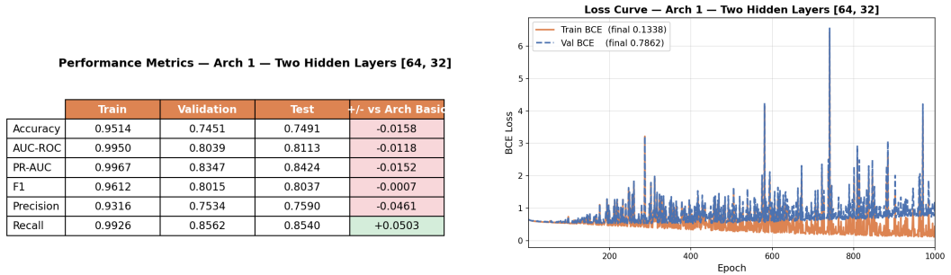
Figure 6.18: Architectural Iteration 1
