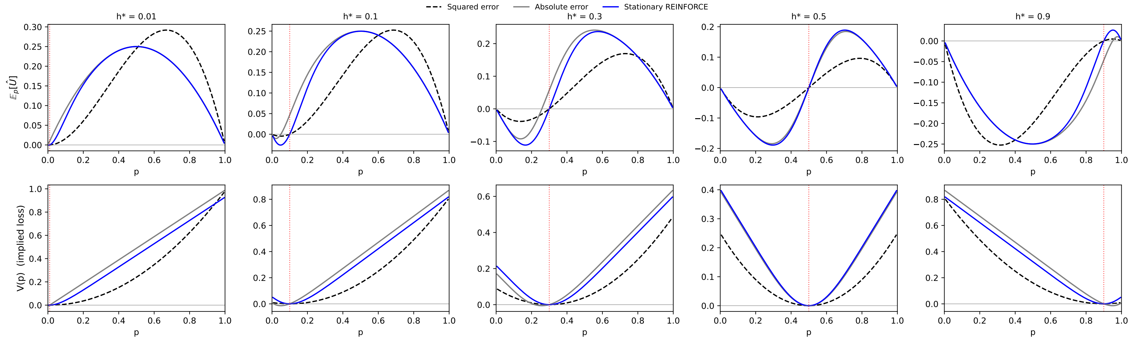
Expected gradient and implied loss — Bernoulli model, M=16
