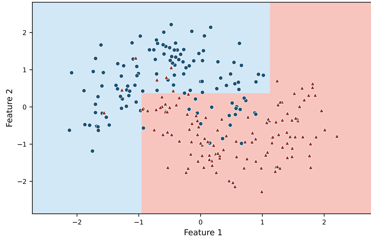
(a) Standard CART Hard binary decision regions
