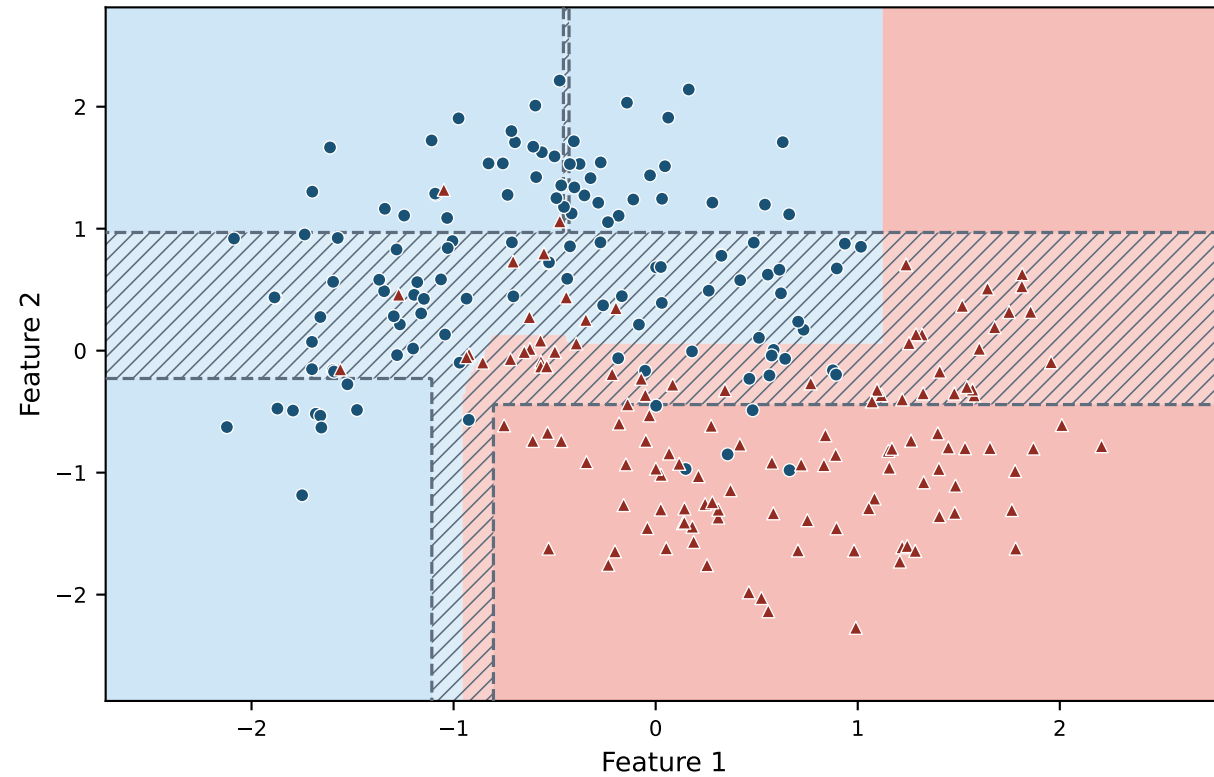
(b) Ternary Decision Tree (Quality-Plateau \delta ) Hatching = boundary-uncertain zone (46.4%) | Decided accuracy: 0.948
