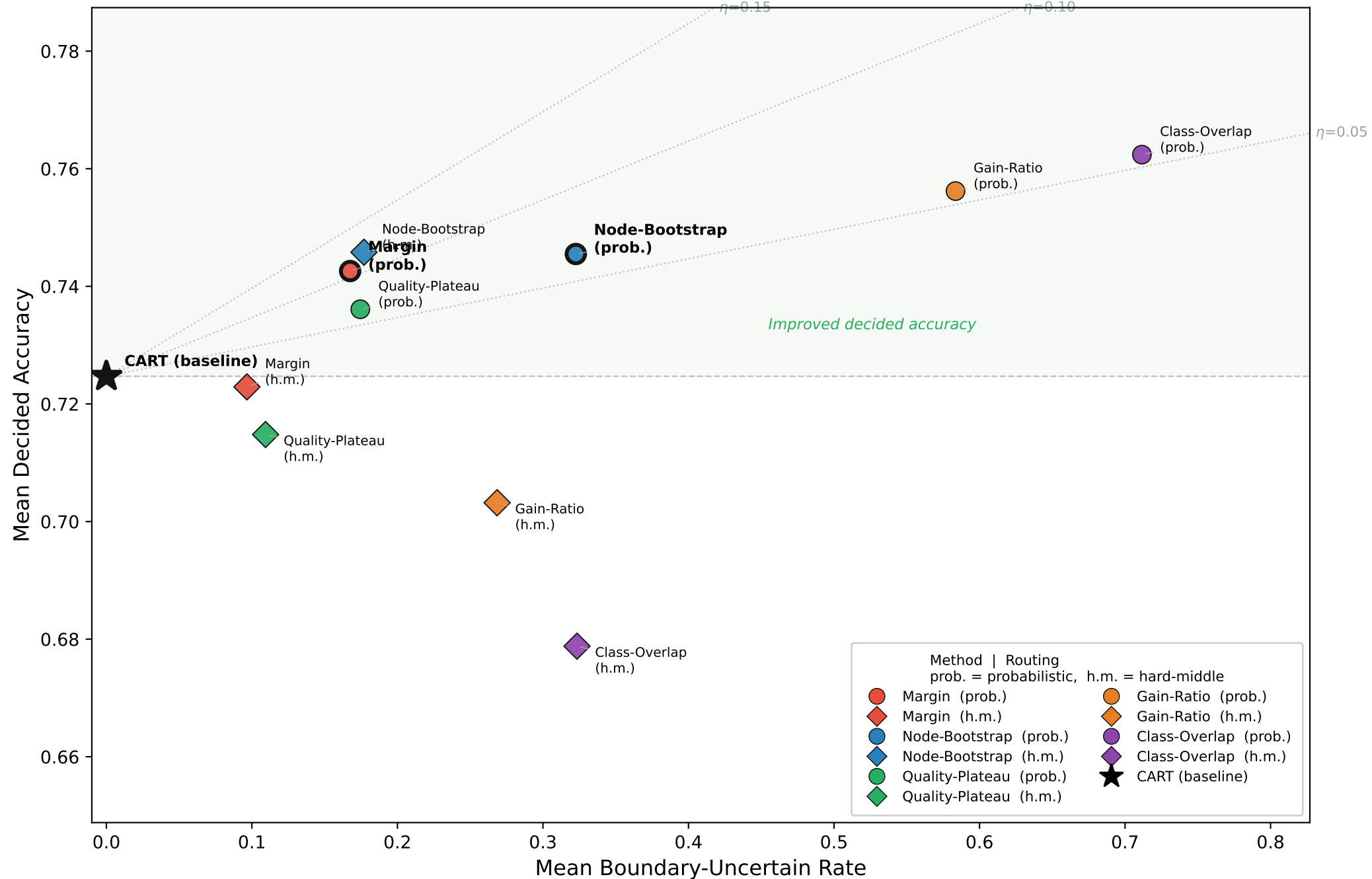
Accuracy-Coverage Tradeoff — All Combinations on OpenML-CC18
