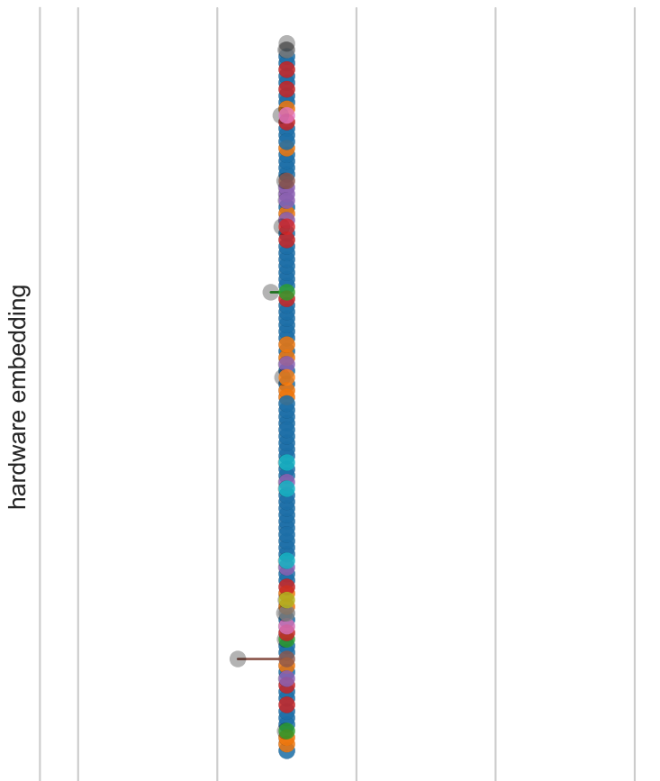
horizon = 1
