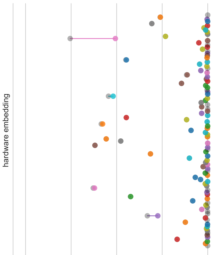
horizon = 4
