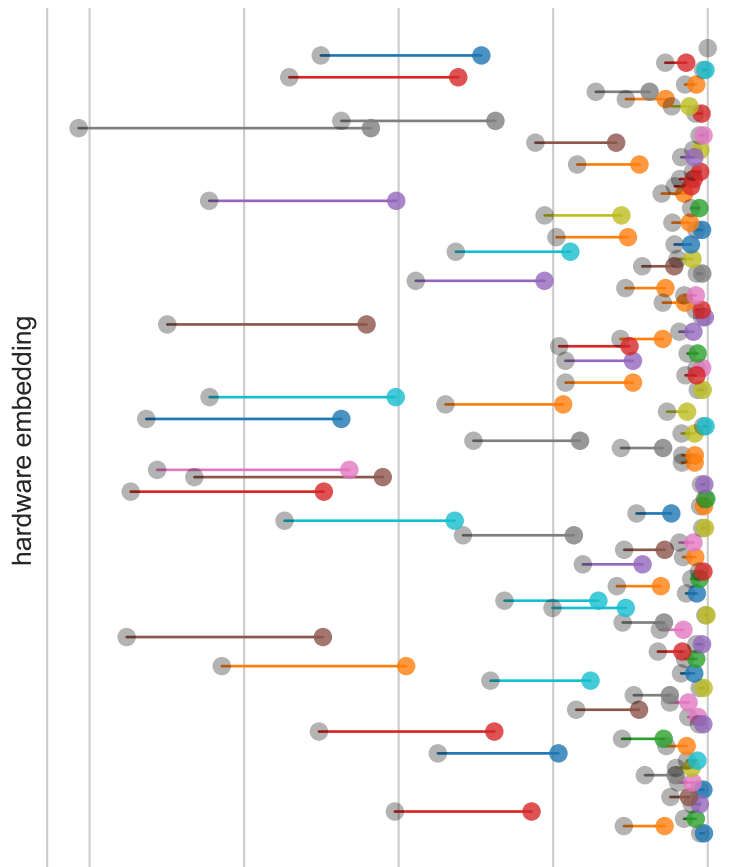
horizon = 3
