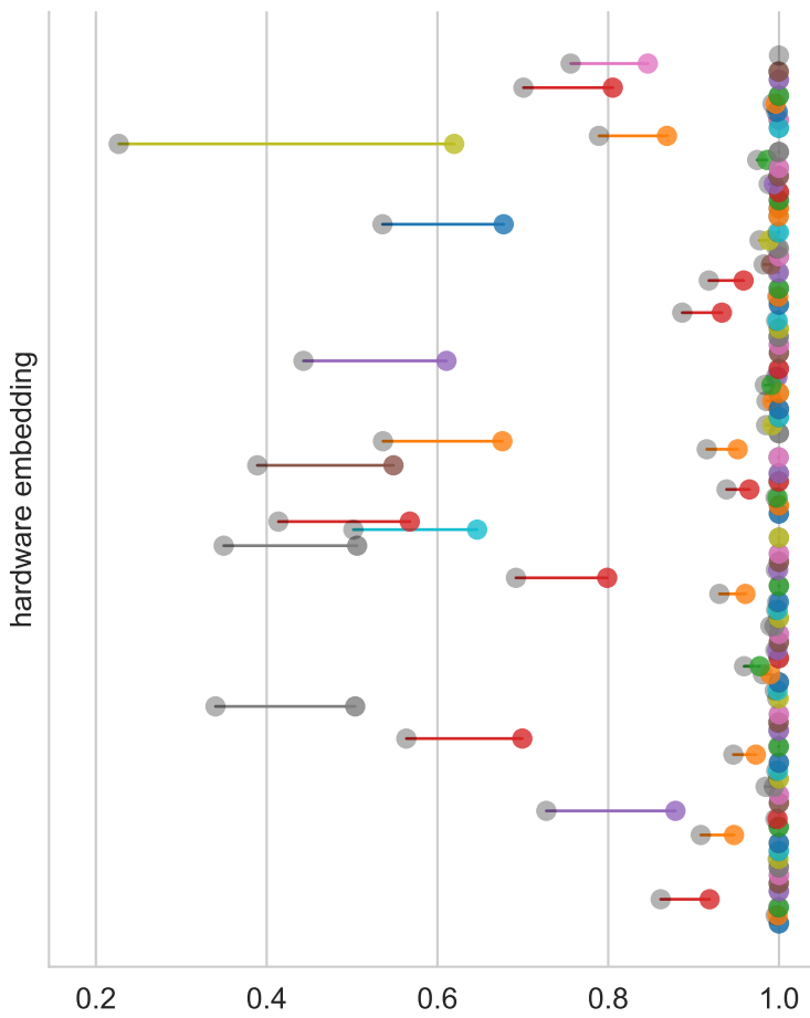
horizon = 7
