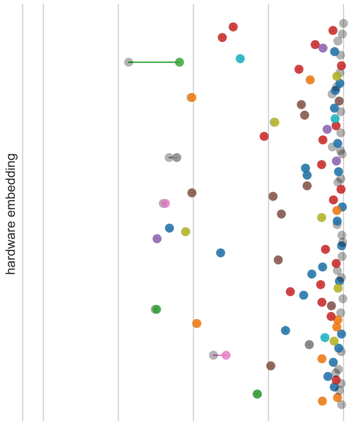
horizon = 2
