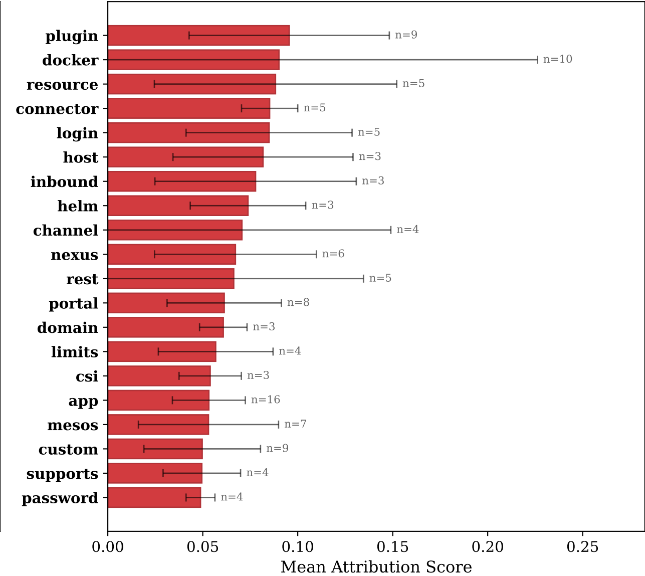
Non-Design Issue Words
