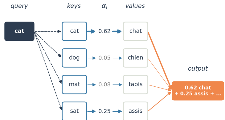
Soft lookup (attention)
