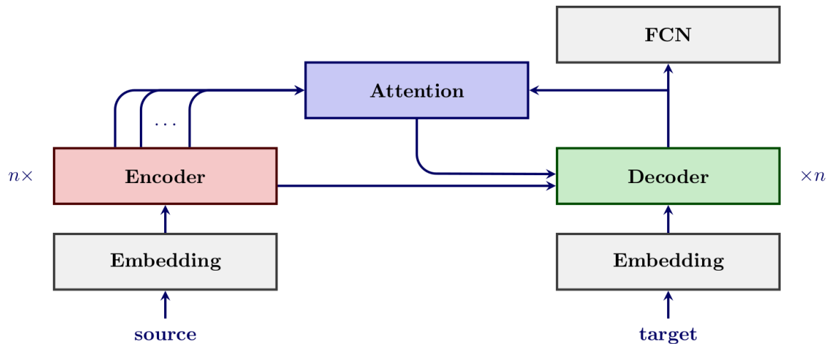
RNN encoder-decoder architecture with the Bahdanau attention mechanism
