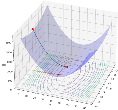
Batch Gradient Descent
