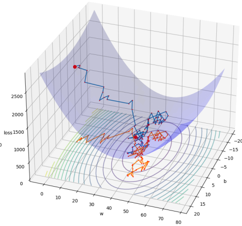
Stochastic Gradient Descent
