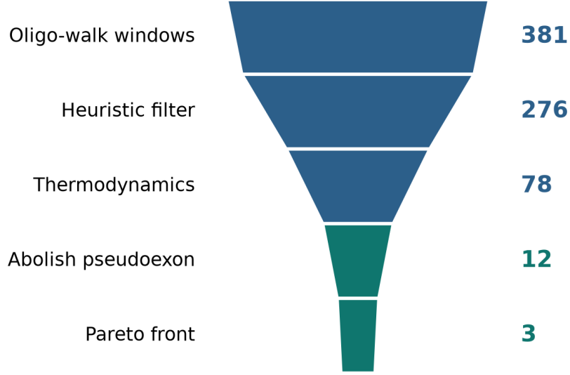
Figure 1: Candidate funnel with the current numbers. The two green stages are the ones that require neural inference; everything upstream is sequence arithmetic. The width of each block scales as n^{0.42} so the last stages remain visible.
