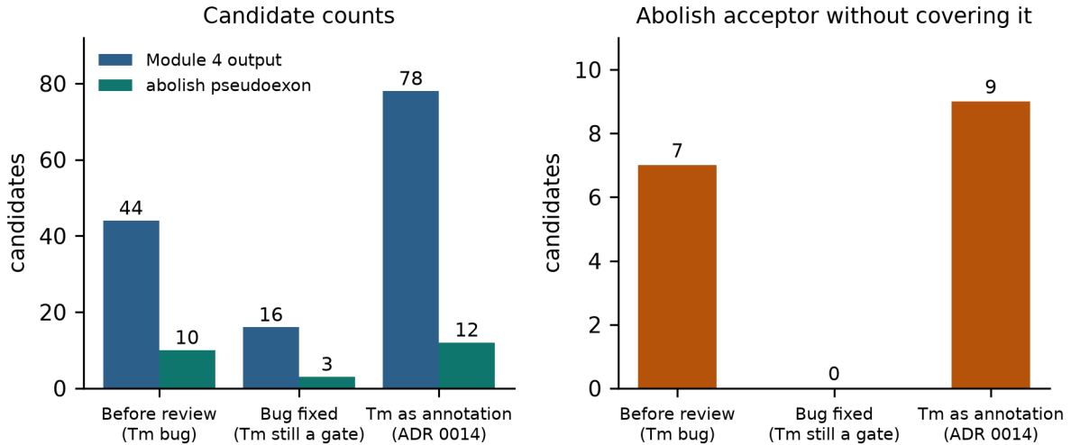
Figure 3: What the review changed. Left: candidates surviving Module 4 and, of those, how many abolish the pseudoexon. Right: candidates that abolish the cryptic acceptor without covering it — the observation that had motivated the project’s verdict criterion. It existed before the review for the wrong reason (a bug), vanished entirely when the bug was fixed, and reappeared on solid ground once T_m stopped being used as a filter.
