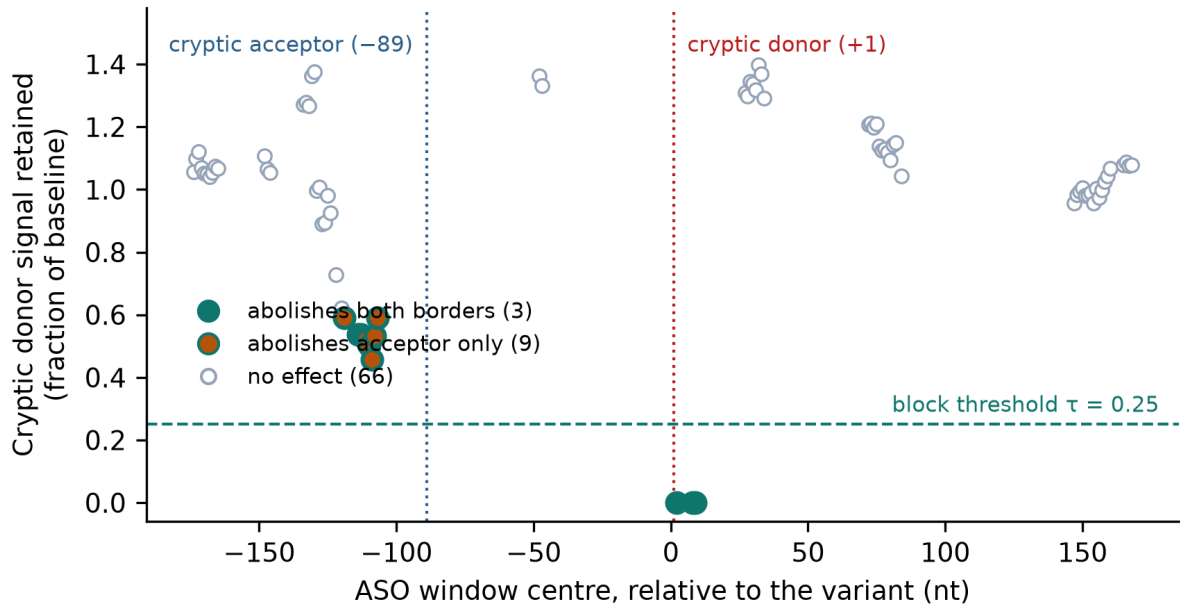
Figure 2: Effect of masking each candidate window on the cryptic donor signal, as a fraction of the unmasked baseline (Equation 1). Windows covering the donor at +1 drive it to zero. Nine candidates centred near -110 abolish the acceptor without covering the donor, and are visible here only as a partial drop in donor signal — their acceptor retention is what Equation 2 evaluates. The dashed line is the declared threshold \tau = 0.25 .
