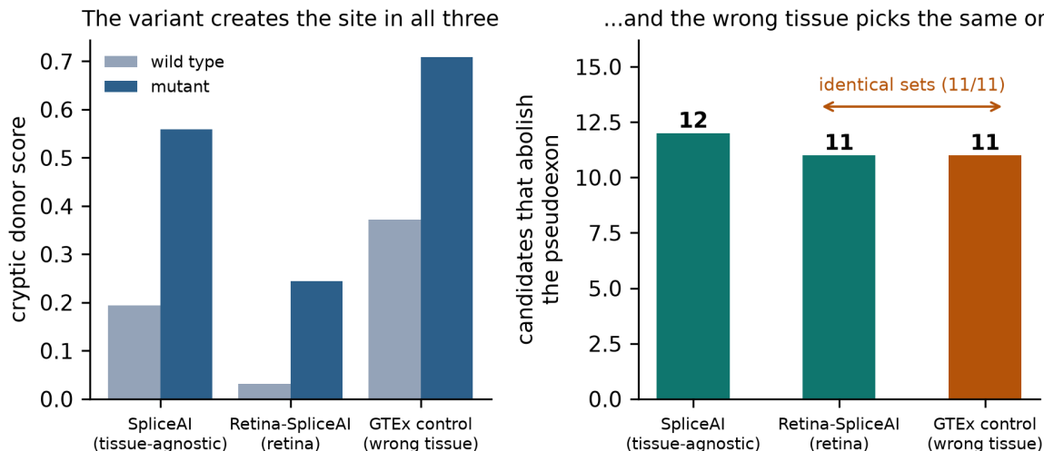
Figure 4: The negative control. Left: all three weight sets — tissue-agnostic, retina-trained, and a GTEx model that deliberately excludes neural retina — agree that the variant creates the cryptic donor, though they disagree on its absolute strength. Right: the retina model and the wrong-tissue model select identical candidate sets (11 of 78); the tissue-agnostic model differs by one. Since the wrong tissue reproduces the result, agreement between them cannot be evidence of tissue-robust biology.
