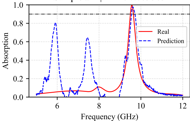
Sample #14|MAE: 0.079363
