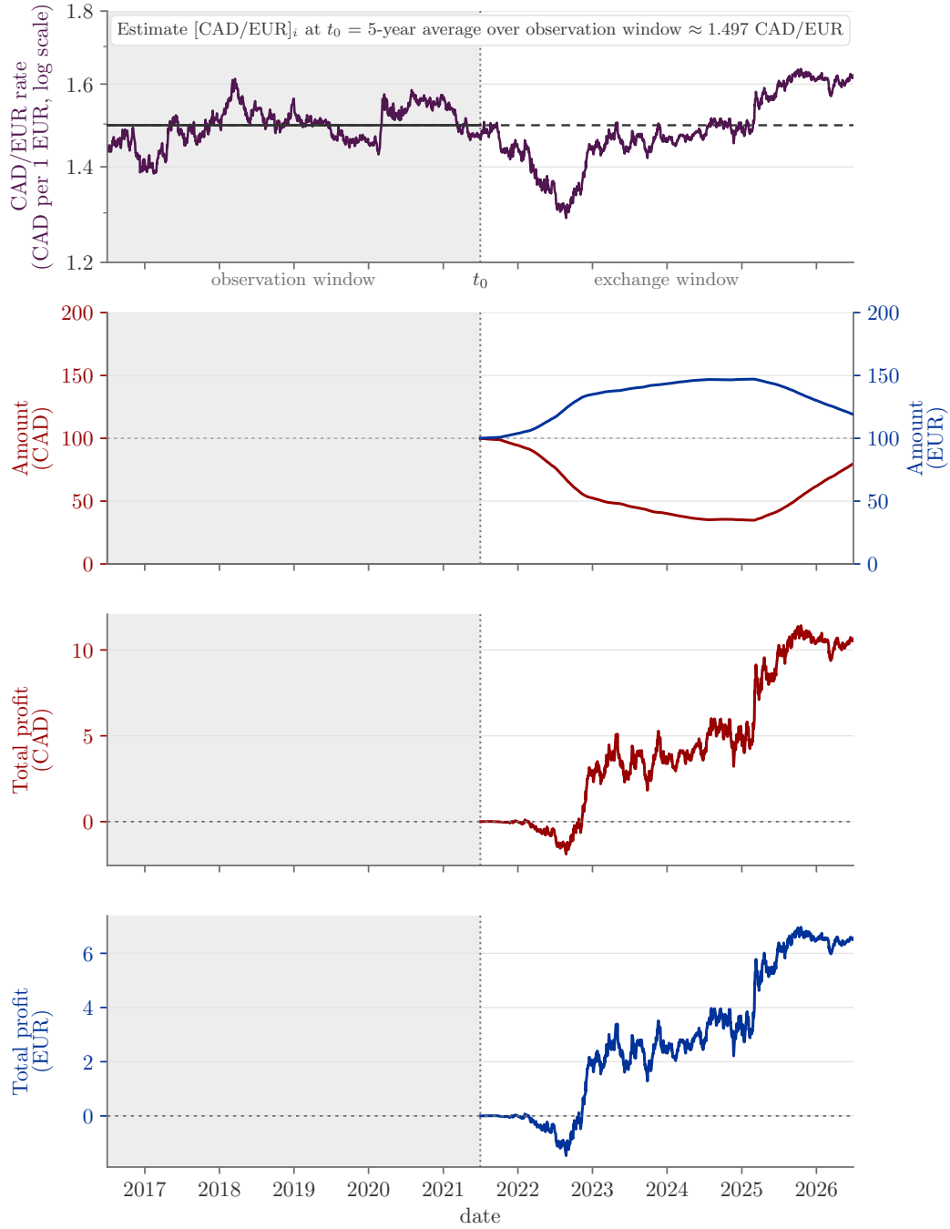
Figure 5: Numerical illustration on real data: the CAD/EUR exchange rate (top, FRED series DEXCAUS [7] and DEXUSEU [8], price on a log axis) over the shaded observation window, 2016-07-01 to 2021-07-01, used only to compute a plain average (solid, horizontal: no trend fit is warranted here) that becomes the declared estimate throughout the unshaded exchange window, 2021-07-01 to 2026-07-01, \approx 1.497 CAD per EUR (dashed line). Second: the two account balances of Alice’s wallet, starting at 100 CAD (red, left axis) and 100 EUR (blue, right axis), each kept in its own native currency. Third and fourth: Alice’s profit since the start of the exchange window (Eqs. (10)–(11)), accounted in CAD ( P^{\text{CAD}} , red) and independently in EUR ( P^{\text{EUR}} , blue) — the same quantity, related exactly by Eq. (12), not two independent findings.
