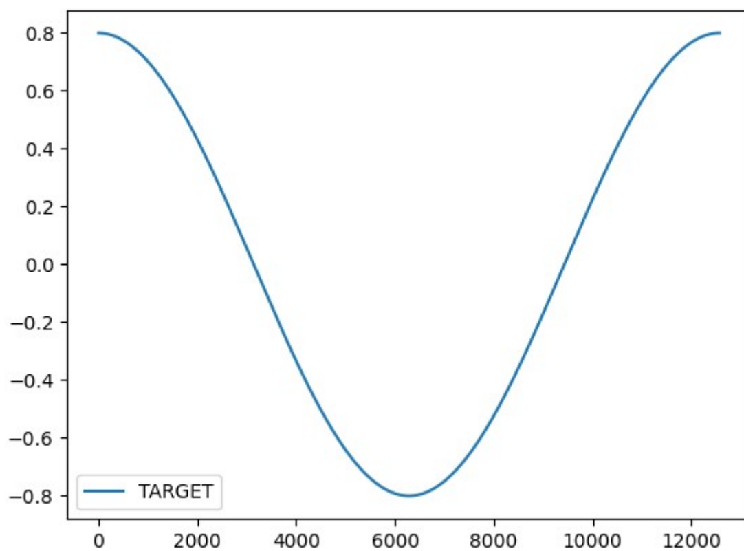
Epochs: 10
