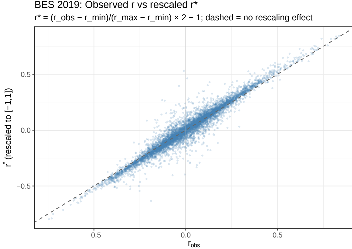
Figure 7: Observed Pearson correlation r_{\text{obs}} versus bound-rescaled correlation r^* for all 7,503 BES 2019 variable pairs. The dashed diagonal marks no rescaling effect ( r^* = r_{\text{obs}} ). Points above the diagonal have been amplified by rescaling; points below have been attenuated.
