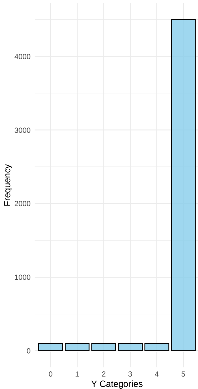
Marginal Distribution of Y
