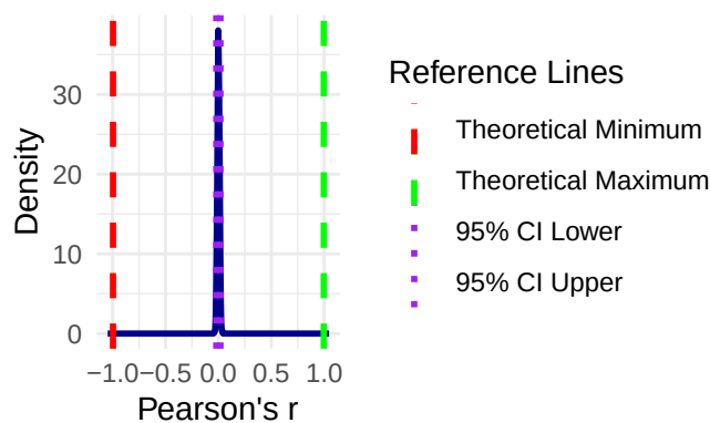
Permutation Distribution – HighlySkewed
