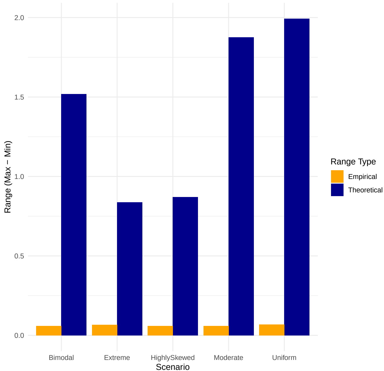
Range of Pearson's r by Marginal Scenario
