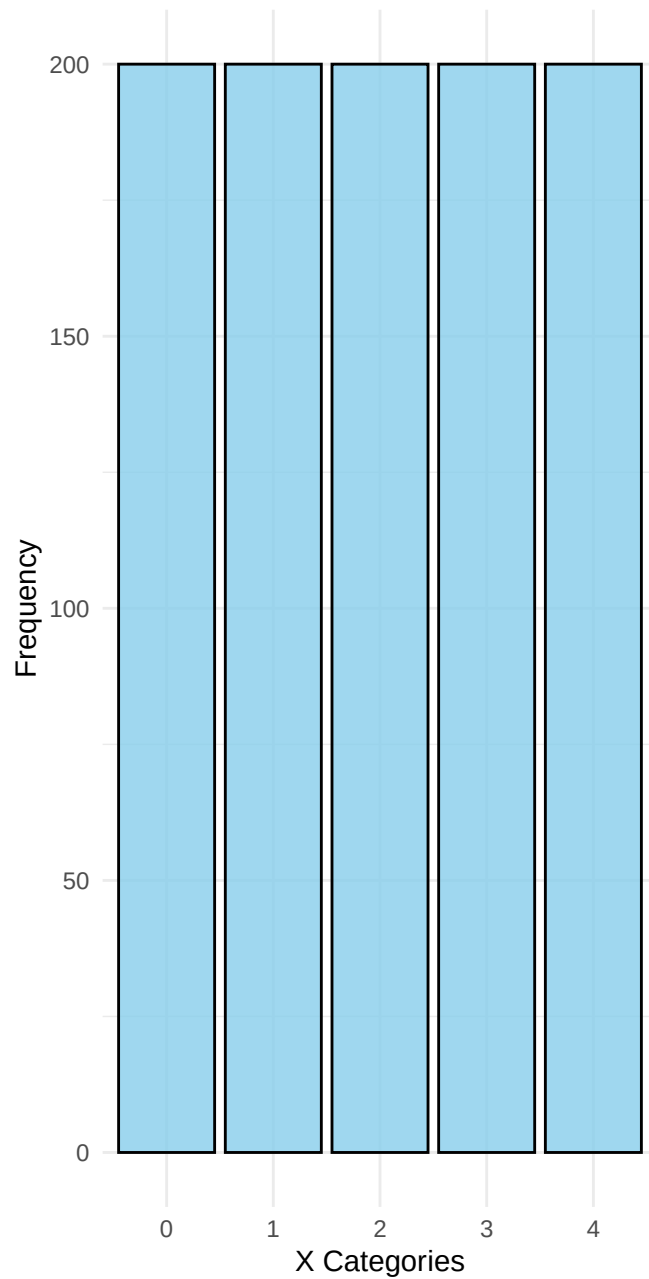
Marginal Distribution of X
