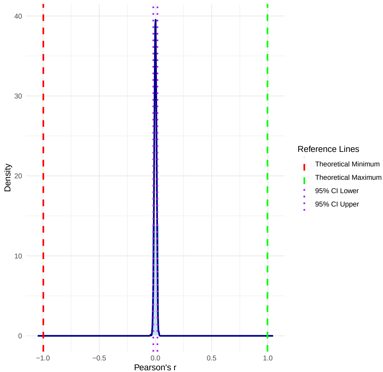
Permutation Distribution (Uniform, n = 10000 )
