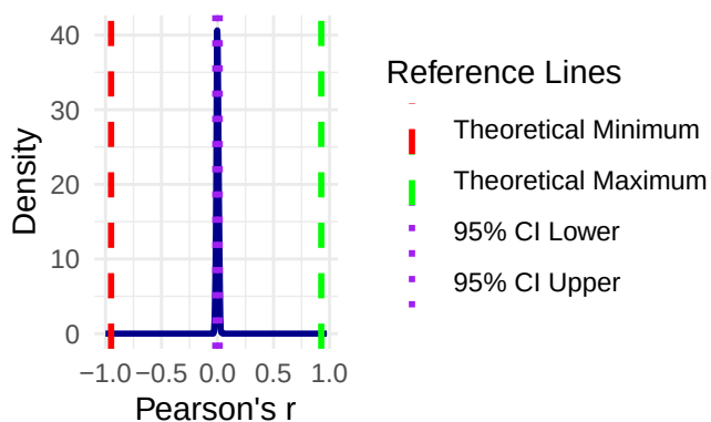
Permutation Distribution – Moderate
