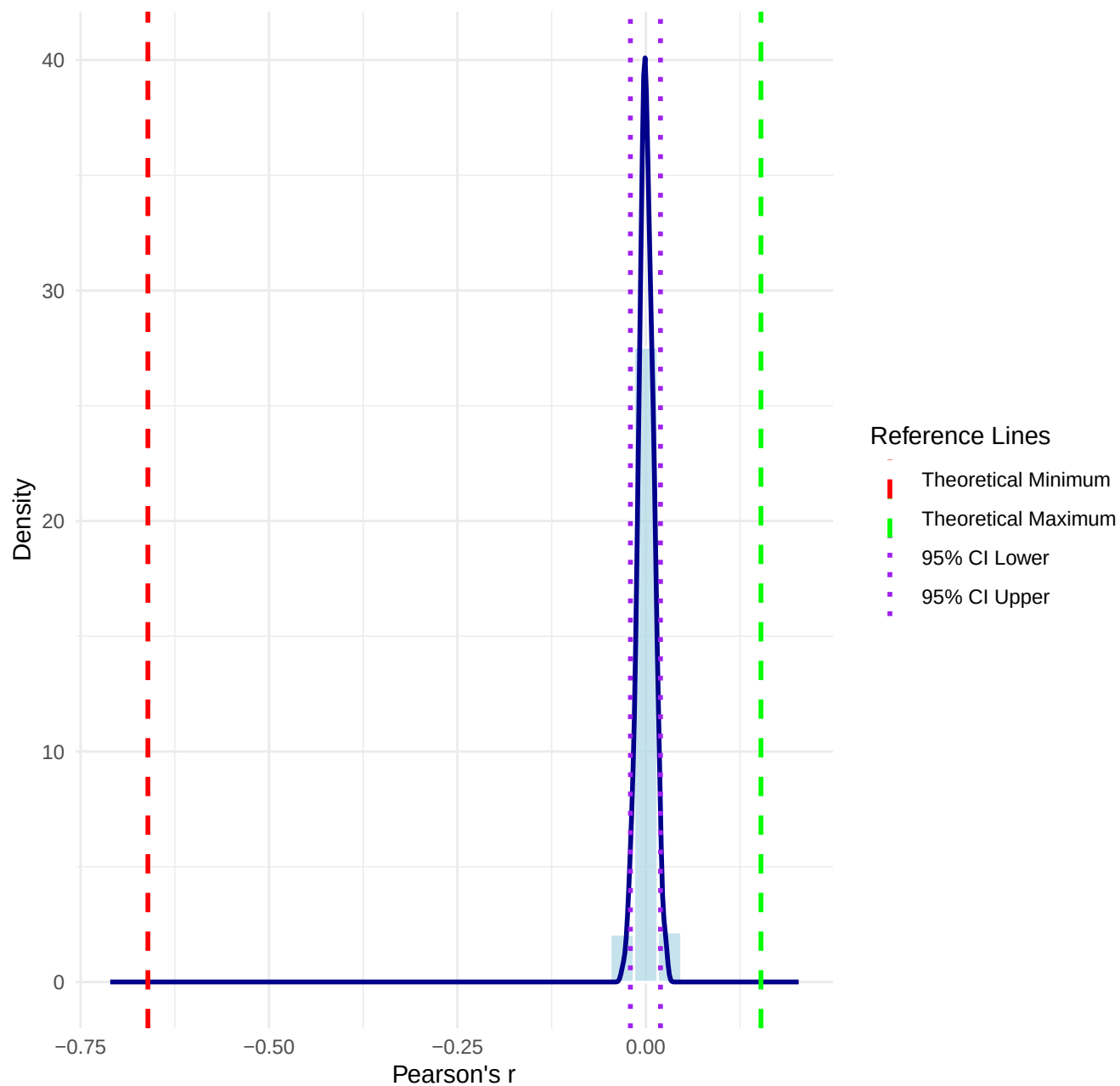
Permutation Distribution (Extreme, n = 10000 )
