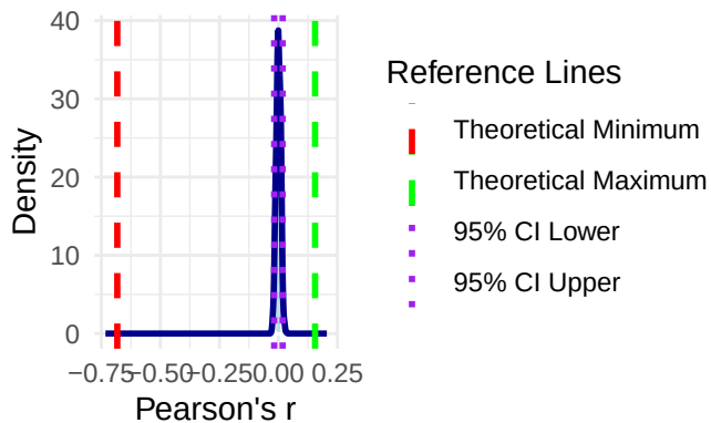
Permutation Distribution – Bimodal
