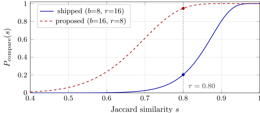
Figure 6: LSH retrieval probability. The decision threshold is \tau = 0.80 ; the shipped banding retrieves only 20.4% of true duplicates there.
