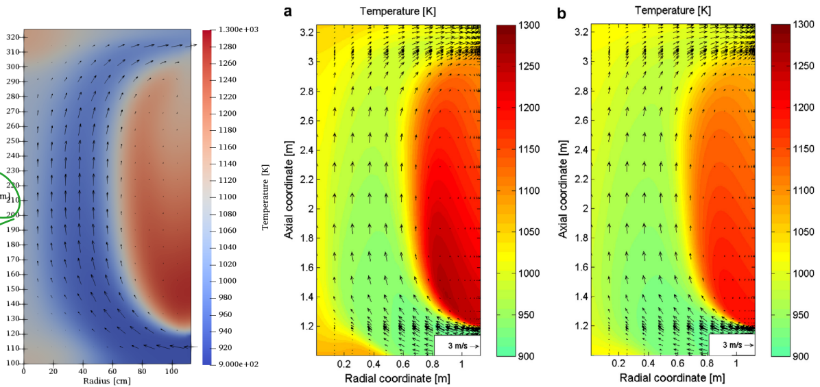
Figure 5.1: Temperature and velocity fields in the core from Moltres (left), Polimi (center), and TUDelft (right) models. The colors represent temperature according to the respective colorbars and the arrows represent velocity fields.
