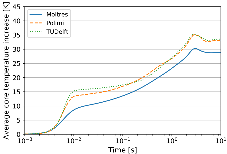
Figure 6.5: Average core temperature increase following a 200 pcm step-wise reactivity insertion in the Moltres, Polimi, and TUDelft models [8].
