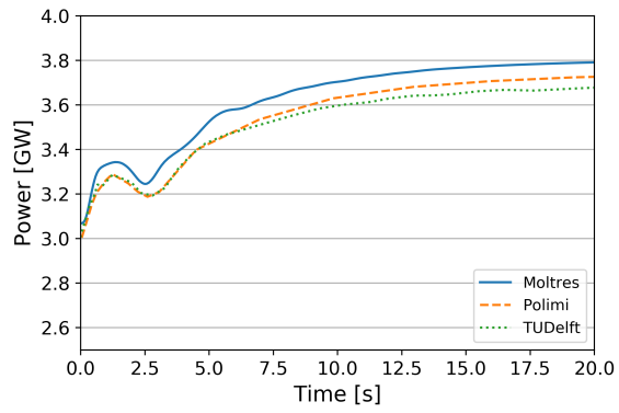
Figure 6.17: The first 20 s of the power output and average core temperature increase during an unprotected pump overspeed transient.
