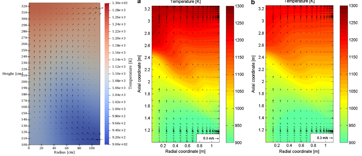
Figure 6.14: Temperature and velocity fields in the core at t = 300 s during a loss of flow transient in the Moltres ( \mu_c = \frac{1}{2}\mu_{t,0} ), Polimi, and TUDelft models.
