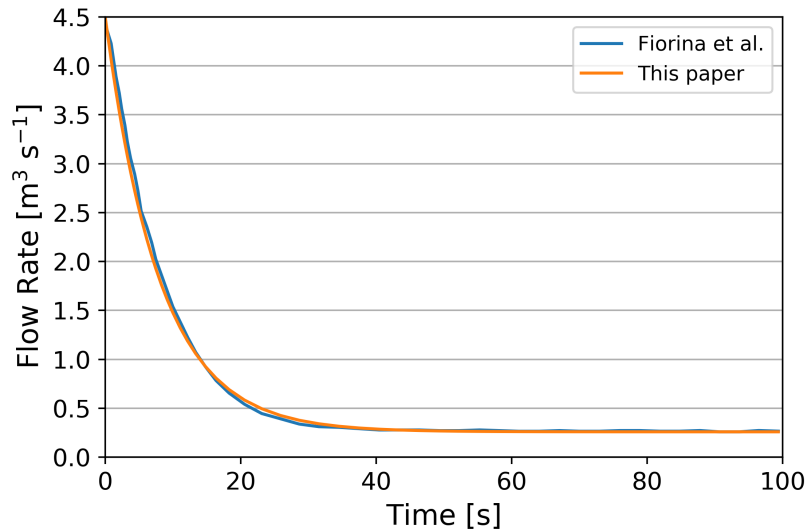
Figure 6.11: The change in flow rate in the Polimi and TUDelft models and the imposed flow rate in Moltres.
