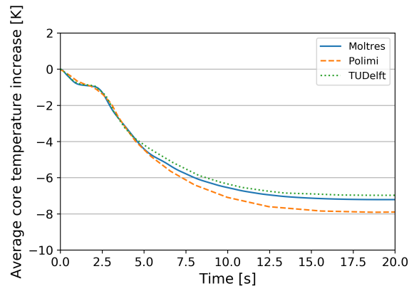
Figure 6.17: The first 20 s of the power output and average core temperature increase during an unprotected pump overspeed transient.
