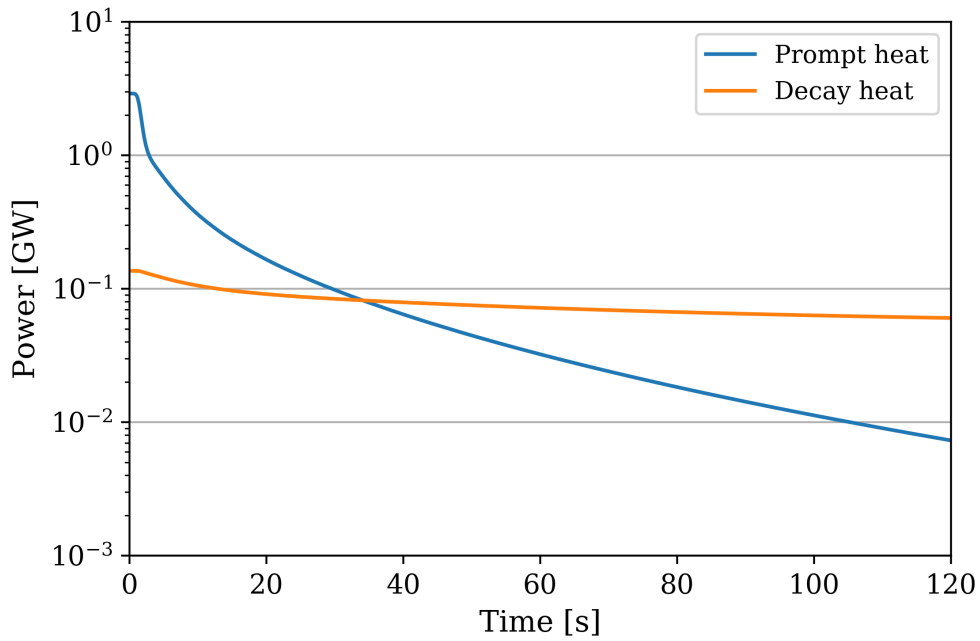
Figure 6.8: Power output during an unprotected loss of heat sink transient in the Moltres model with and without decay heat.
