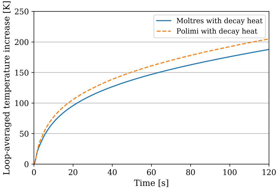
Figure 6.10: Loop-averaged temperature increase during an unprotected loss of heat sink transient in the Moltres and Polimi models [8] with decay heat.
