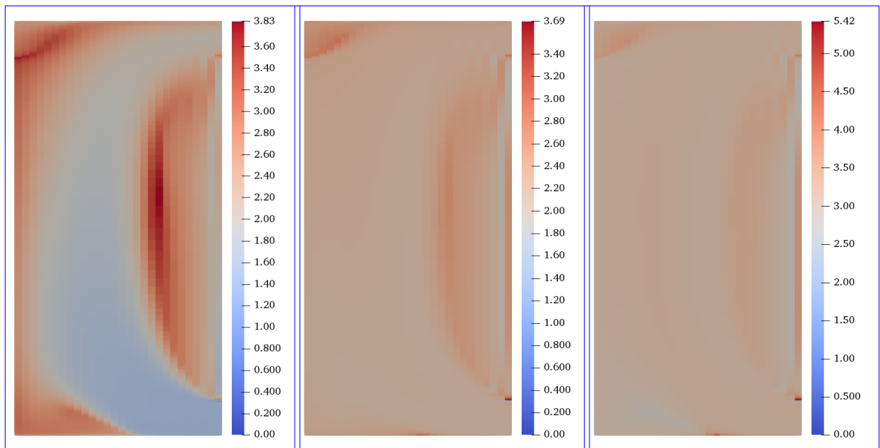
Figure 5.7: Decay heat source distribution in the core for decay heat groups 1 to 3 (from left to right). Refer to Figure 5.8 for the height and radius scales on the y and x axes, respectively. Note the different scales for each distribution.
