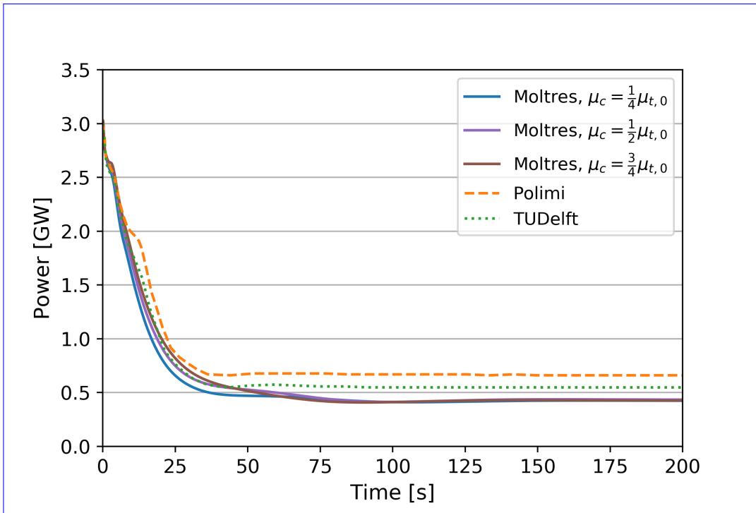
Figure 6.16: Power output during an unprotected pump overspeed loss of flow transient in the Moltres, Polimi, and TUDelft models [9].
