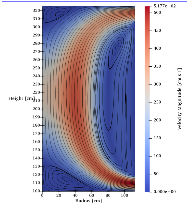
Figure 5.2: Fuel salt flow streamlines and velocity magnitude in the core. The colors represent velocity magnitude according to the color bar on the right.
