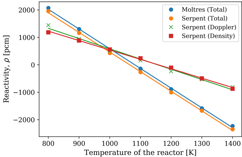
Figure 4.1: Reactivity values from Serpent and Moltres. The Doppler reactivity values were calculated at a fixed density of 4.1249 g cm -3 . The density thermal expansion reactivity values were calculated at a fixed temperature of 973 K.
