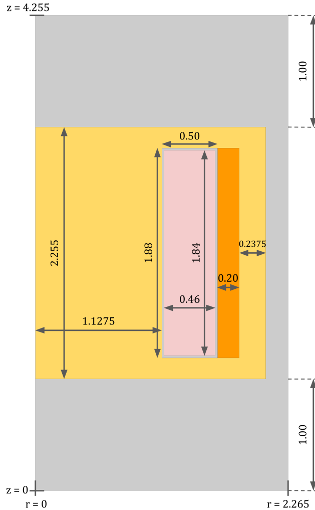
Figure 2.2: 2-D axisymmetric model of the MSFR core used for the simulations in Serpent. All dimensions are in meters. [47]
