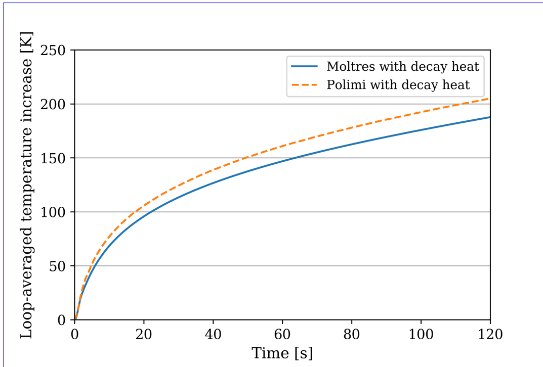
Figure 6.11: Loop-averaged temperature increase during an unprotected loss of heat sink transient in the Moltres and Polimi models [9] with decay heat.
