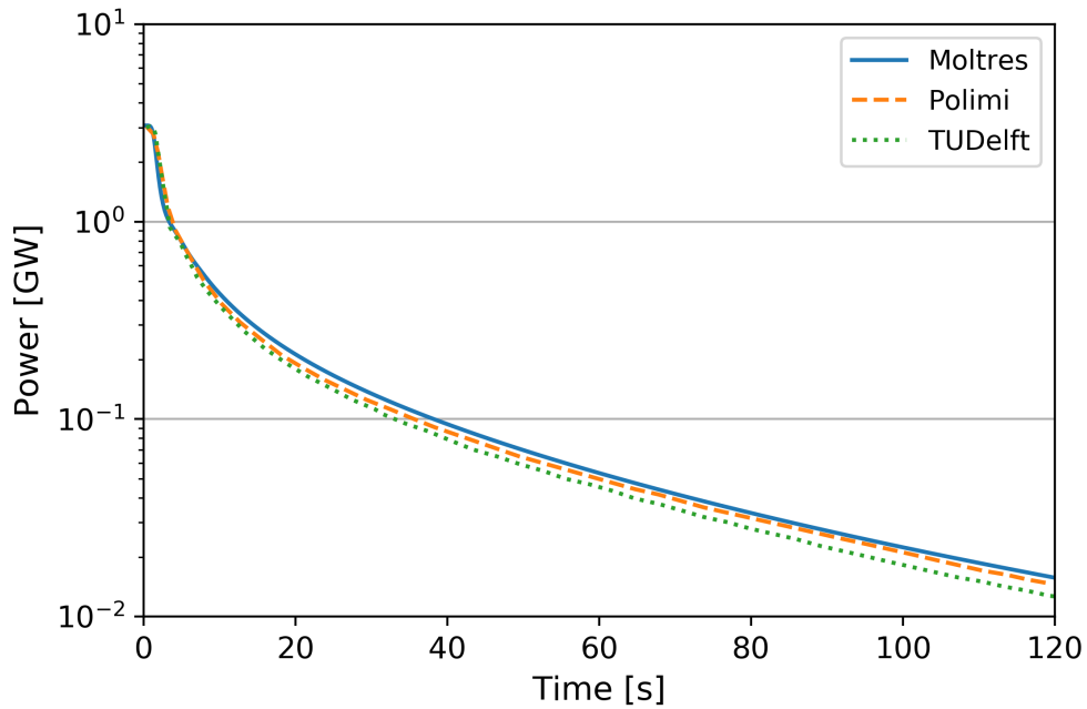
Figure 6.7: Power output during an unprotected loss of heat sink transient in the Moltres, Polimi, and TUDelft models [9] without decay heat.
