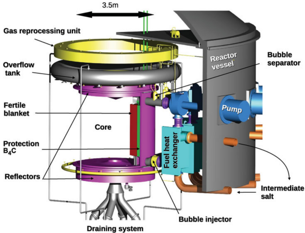
Figure 2.1: Schematic view of the MSFR concept. Figure reproduced from Brovchenko et al. [30].
