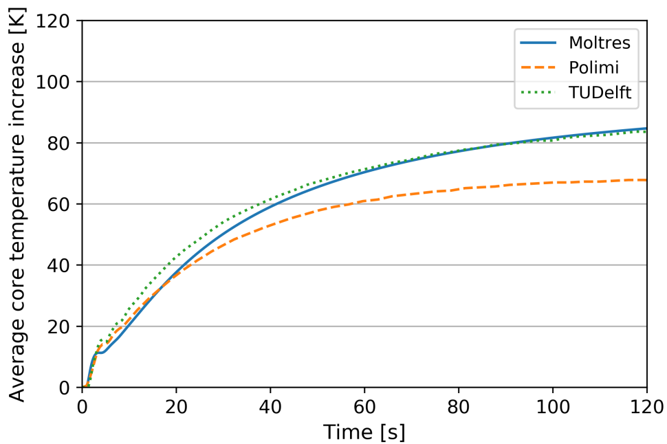
Figure 6.8: Average core temperature increase during an unprotected loss of heat sink transient in the Moltres, Polimi, and TUDelft models [9] without decay heat.
