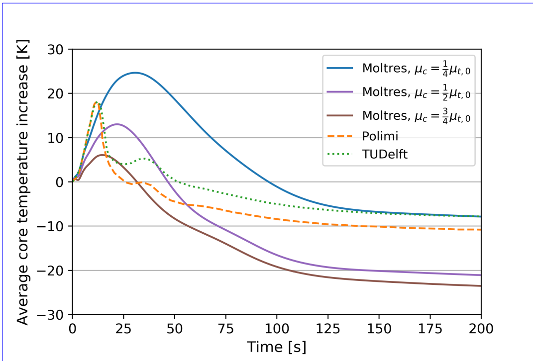
Figure 6.17: Average core temperature increase during an unprotected pump overspeed loss of flow transient in the Moltres, Polimi, and TUDelft models [9].
