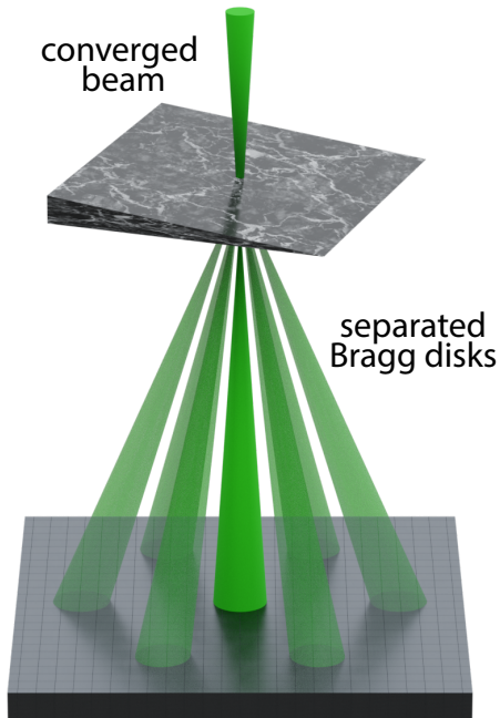
nanobeam 4D-STEM
