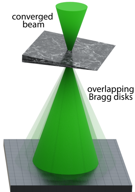
large convergence angle 4D-STEM
