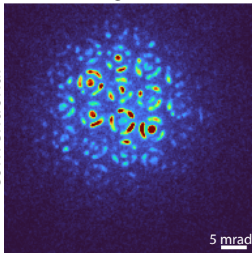
single DP
