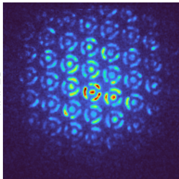
MAPED
