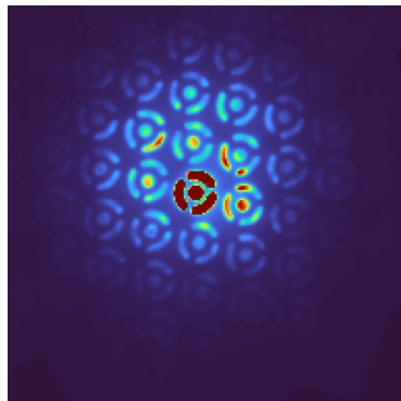
mean DP
