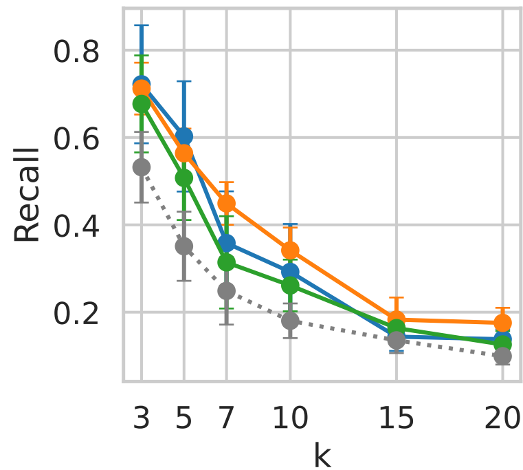
Recall
