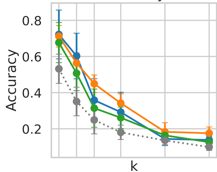
Accuracy
