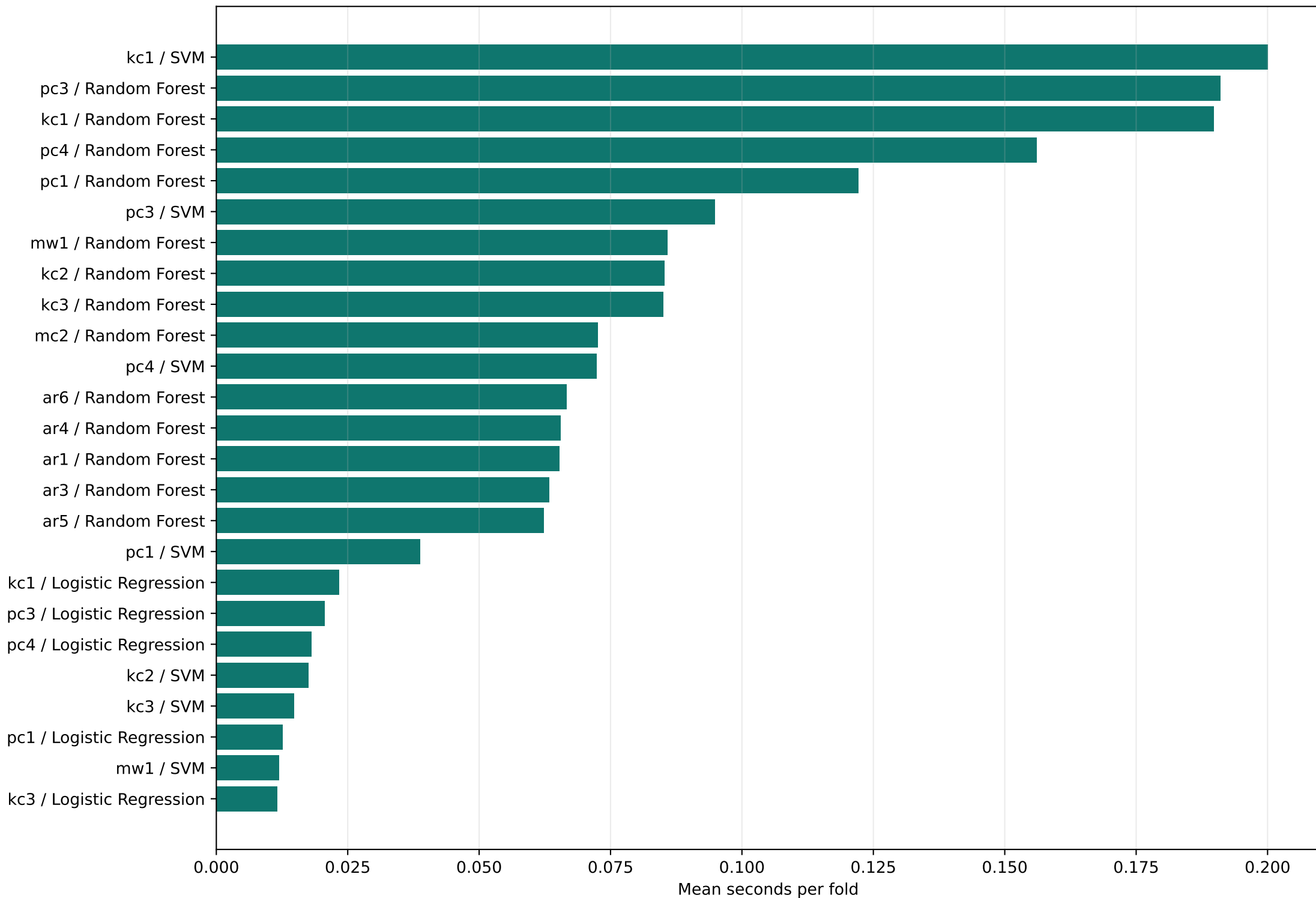
Slowest Dataset/Model Fold Runtimes
