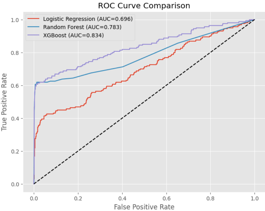
Figure 6.2: ROC Curve Comparison of Baseline Models
