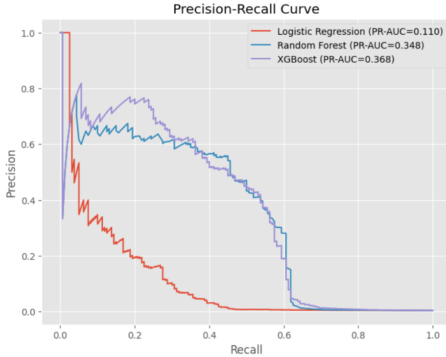
Figure 6.3: Precision–Recall Curve Comparison
