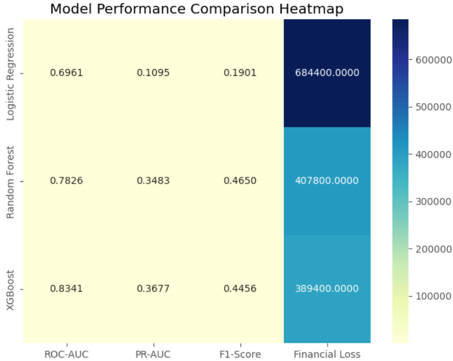
Figure 6.4: Model Performance Comparison Heatmap
