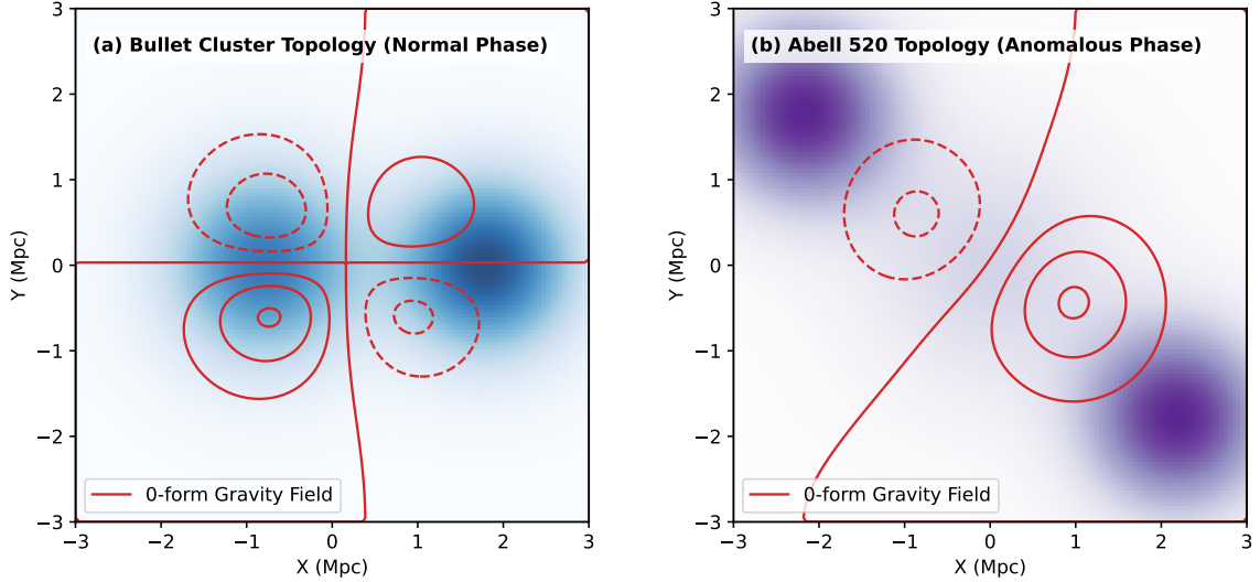
Figure 2: The topological bifurcation profiles of cluster merger dynamics mapped directly from the multi-grid validation solver tree. (a) The normal separation phase in the Bullet Cluster proxy context, where the unrendered 0-form gravity skeleton field (red contours) systematically outruns the stripped baryonic gas flow (blue fill), qualitatively reproducing the separation pattern observed in weak-lensing reconstructions of the Bullet Cluster. (b) The anomalous core-retention phase in the Abell 520 configuration, capturing the central localized dark potential trapping induced by isotropic disordered momentum flux cancellation. Note that the fluid backgrounds are synthetic, idealized profiles constructed for structural reference rather than full hydrodynamical coupling solutions.
