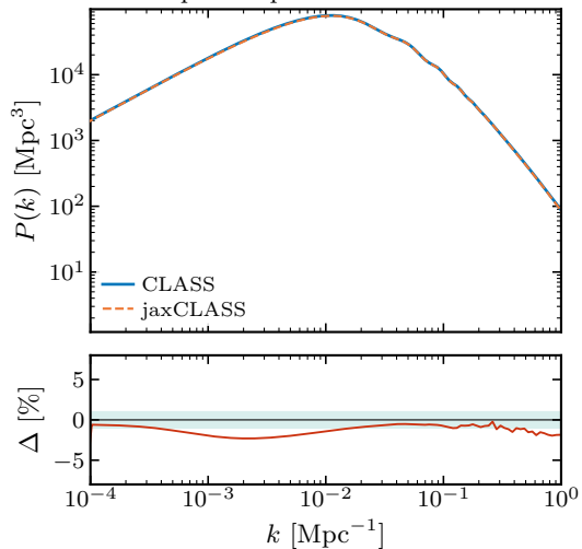
Matter power spectrum
