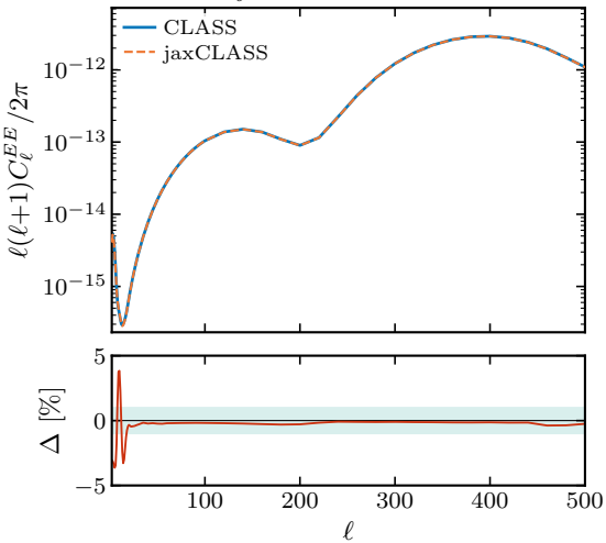
E -mode C_\ell^{EE}
