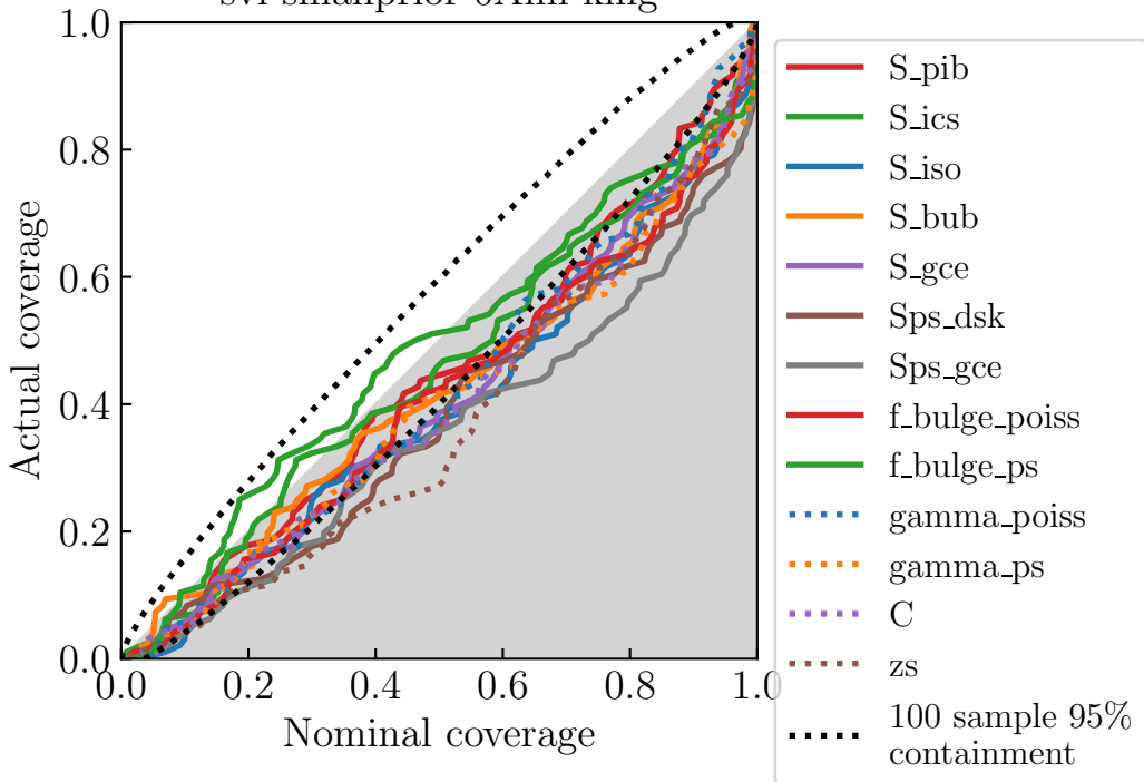
svi-smallprior-0Alm-king
