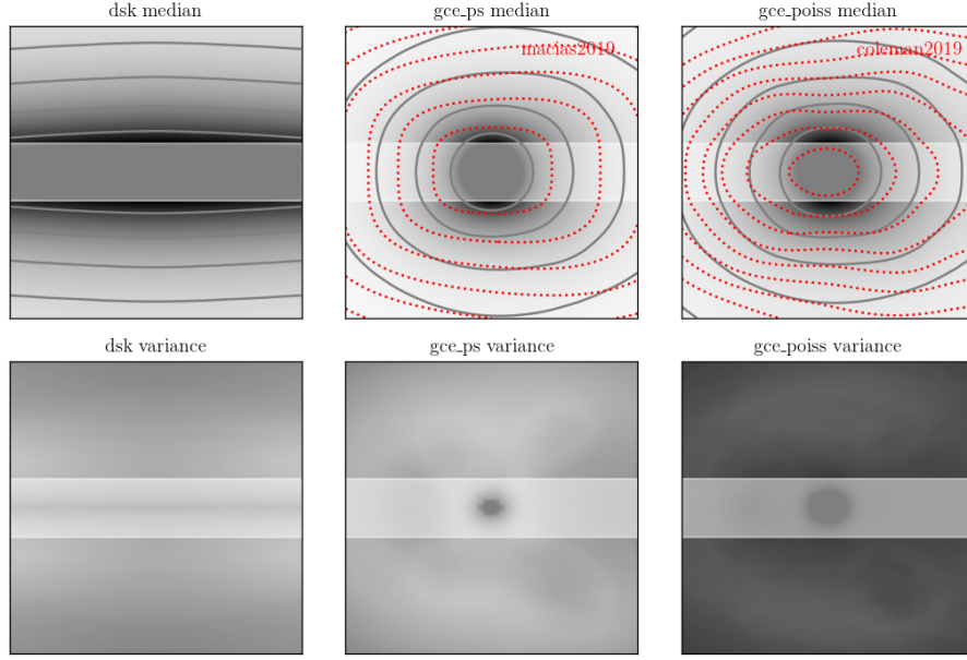
Figure 1. Summaries of the inferred posteriors for disk-correlated PS, GCE-correlated PS, and GCE-correlated smooth emission morphologies. The top row shows the median inferred pixel-wise morphologies, which the bottom row shows the relative middle-68% deviation of the posterior from the median. For comparison, contours for the best-fitting bulge description are shown for the GCE PS and smooth components.
