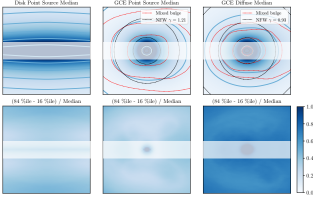
Figure 2. Summaries of the inferred posteriors for disk-correlated PS, GCE-correlated PS, and GCE-correlated smooth emission morphologies from a preliminary analysis of Fermi -LAT data. The top row shows the median inferred pixel-wise morphologies, which the bottom row shows the relative middle-68% deviation of the posterior from the median. For comparison, contours for the best-fitting bulge and DM (NFW) description are shown for the GCE PS and smooth components.
