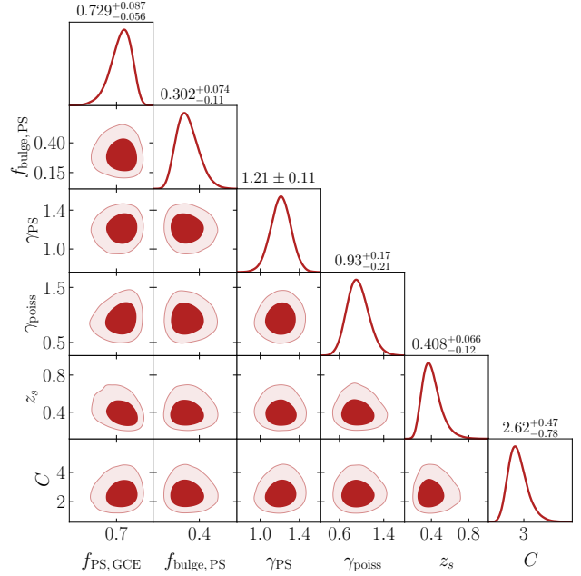
Figure 3. Posteriors on select parameters characterizing the GCE and disk PS morphologies obtained with a preliminary analysis of Fermi -LAT data in the Inner Galaxy. The PS fraction of the GCE f_{\text{PS,GCE}} , the bulge fraction within the PS components f_{\text{bulge,PS}} , distributions on the NFW inner slopes \gamma for the PS and smooth NFW profiles, as well as select parameters characterizing the disk morphology are shown.
