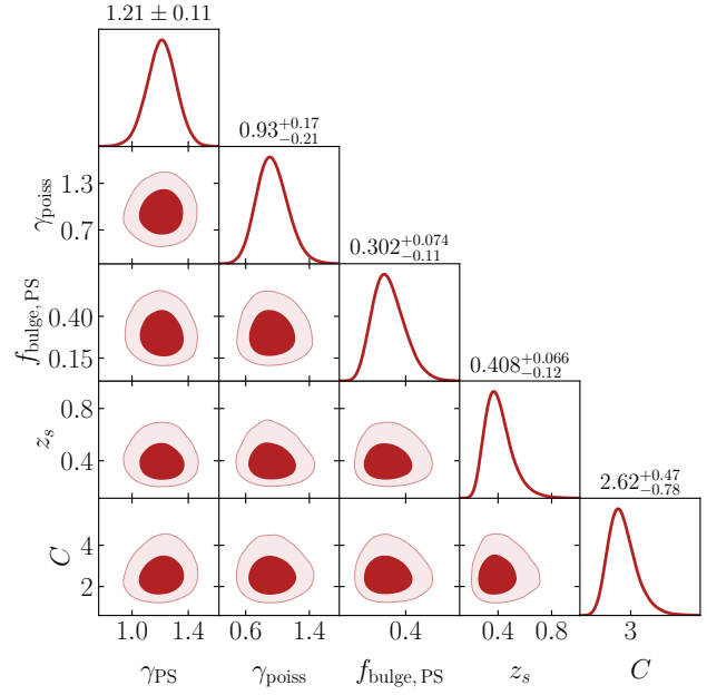
Figure 3. Posteriors on select parameters characterizing the GCE and disk PS morphologies obtained by analyzing Fermi -LAT data in the Inner Galaxy. The bulge fraction f_{\text{bulge,PS}} , distributions on the NFW inner slopes \gamma for the PS and smooth NFW profiles, as well as select parameters characterizing the disk morphology are shown. [SM: Update with PS fraction posterior]
