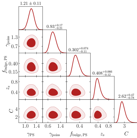
Figure 3. Posteriors on select parameters characterizing the GCE and disk PS morphologies obtained by analyzing Fermi -LAT data in the Inner Galaxy. The bulge fraction f_{\text{bulge}} , distributions on the NFW inner slopes \gamma for the PS and smooth NFW profiles, as well as select parameters characterizing the disk morphology are shown.
