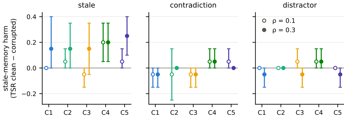
D1, paired bootstrap 95% CI clustered by arc
