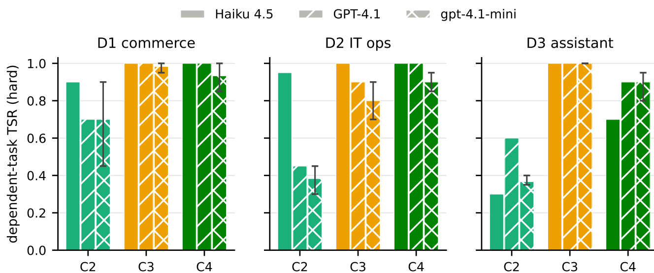
Fig. 6. Hard-tier TSR across agent models (bar hatch = model, color = condition; whiskers = min-max across the 3 gpt-4.1-mini seeds). Embedding retrieval (C2) collapses somewhere for every model, but where is model-idiosyncratic; LLM summarization (C3) is robust everywhere.
