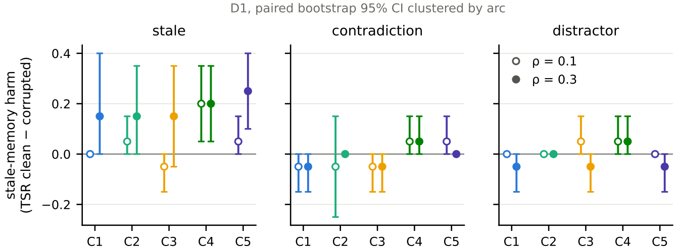
Fig. 4. Stale-memory harm (TSR clean — corrupted, dependent tasks, D1, real implementations) by condition, corruption mode, and corruption rate p ; error bars are paired bootstrap 95% CIs clustered by arc.
