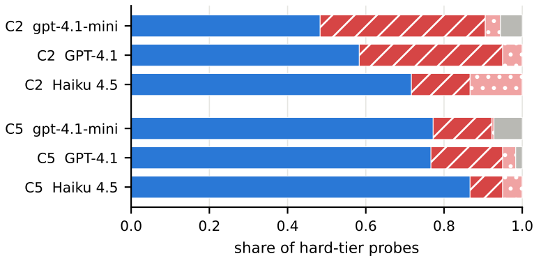
(a) outcome of updated-fact probes
