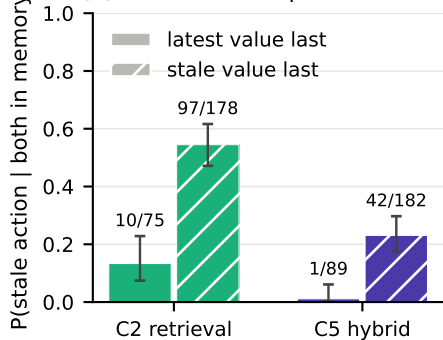
(b) which value is positioned last
