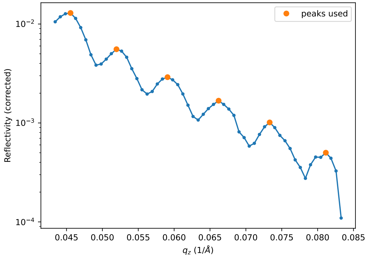
Peak selection for thickness estimate
