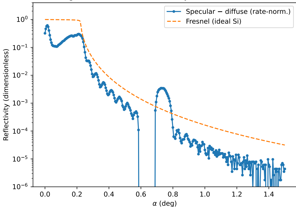
Background-subtracted reflectivity with Fresnel reference
