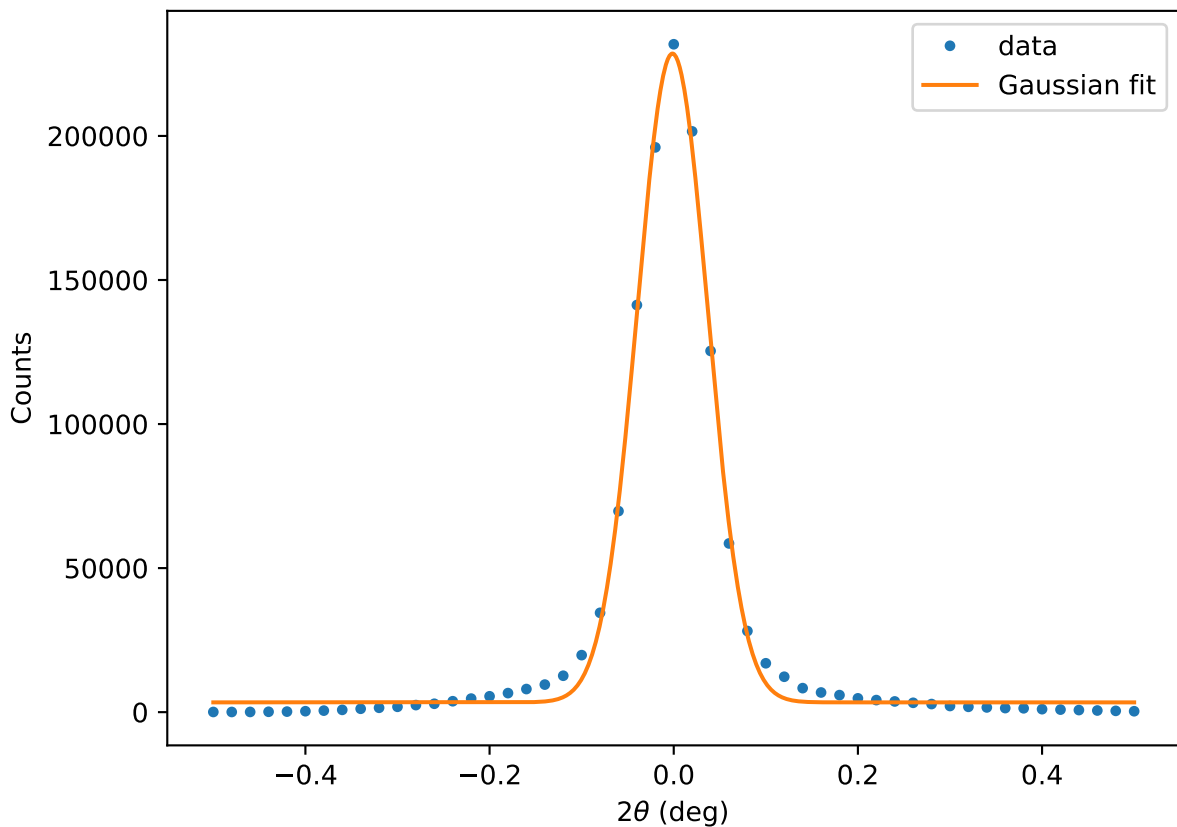
Detector scan: Gaussian fit
